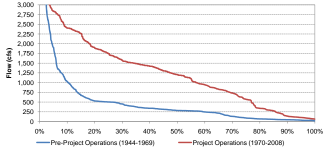
Exceedance Probability of Historical Mean Daily Yuba River Flow at Marysville Before and After Completion of the YRDP for August
