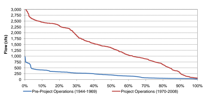
Exceedance Probability of Historical Mean Daily Yuba River Flow at Marysville Before and After Completion of the YRDP for September
