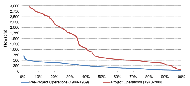
Exceedance Probability of Historical Mean Daily Yuba River Flow at Marysville Before and After Completion of the YRDP for October
