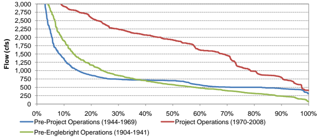
Exceedance Probability of Historical Mean Daily Yuba River Flow at Smartville Before and After Completion of Englebright Dam and the YRDP for August
