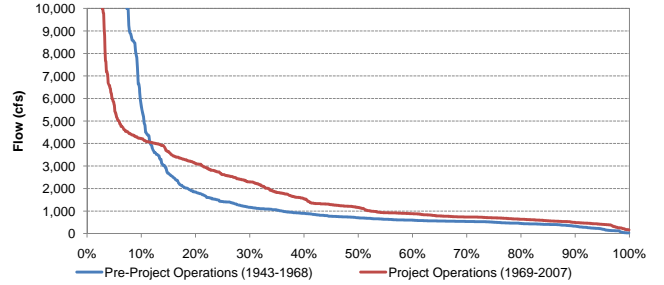
Exceedance Probability of Historical Mean Daily Yuba River Flow at Marysville Before and After Completion of the YRDP for the Full Period of Record
