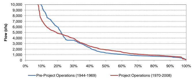
Exceedance Probability of Historical Mean Daily Yuba River Flow at Marysville Before and After Completion of the YRDP for February
