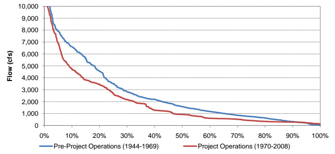
Exceedance Probability of Historical Mean Daily Yuba River Flow at Marysville Before and After Completion of the YRDP for July
