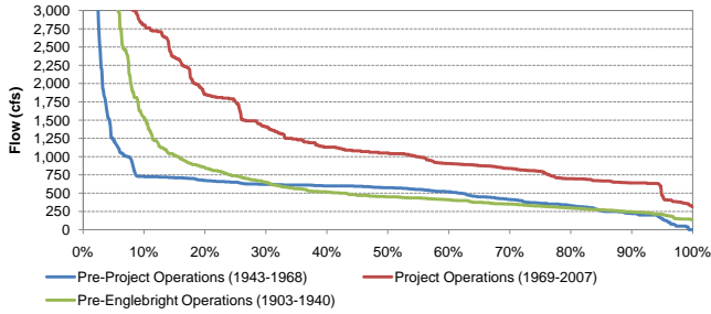
Exceedance Probability of Historical Mean Daily Yuba River Flow at Smartville Before and After Completion of Englebright Dam and the YRDP for December
