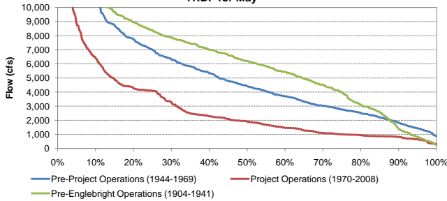
Exceedance Probability of Historical Mean Daily Yuba River Flow at Smartville Before and After Completion of Englebright Dam and the YRDP for May
