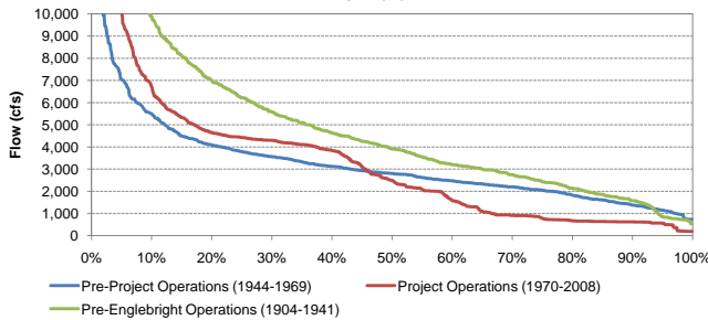
Exceedance Probability of Historical Mean Daily Yuba River Flow at Smartville Before and After Completion of Englebright Dam and the YRDP for April
