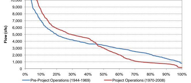
Exceedance Probability of Historical Mean Daily Yuba River Flow at Marysville Before and After Completion of the YRDP for April
