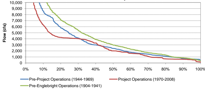
Exceedance Probability of Historical Mean Daily Yuba River Flow at Smartville Before and After Completion of Englebright Dam and the YRDP for March
