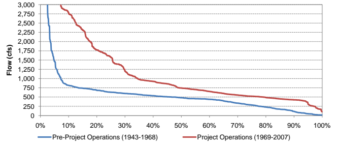
Exceedance Probability of Historical Mean Daily Yuba River Flow at Marysville Before and After Completion of the YRDP for December
