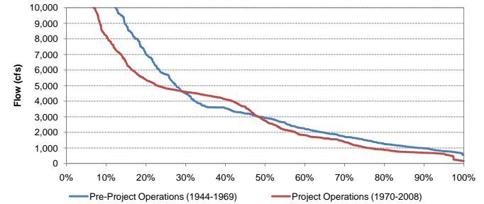
Exceedance Probability of Historical Mean Daily Yuba River Flow at Marysville Before and After Completion of the YRDP for March
