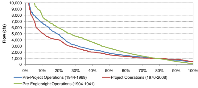
Exceedance Probability of Historical Mean Daily Yuba River Flow at Smartville Before and After Completion of Englebright Dam and the YRDP for July
