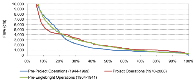
Exceedance Probability of Historical Mean Daily Yuba River Flow at Smartville Before and After Completion of Englebright Dam and the YRDP for February
