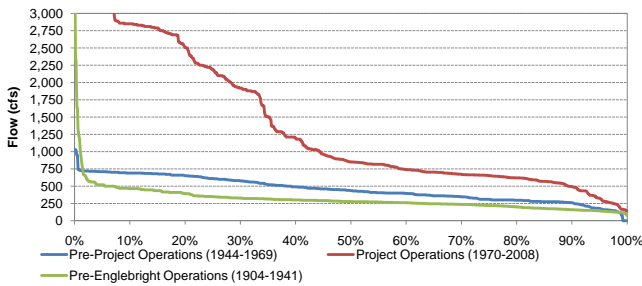
Exceedance Probability of Historical Mean Daily Yuba River Flow at Smartville Before and After Completion of Englebright Dam and the YRDP for October
