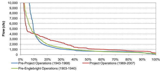
Exceedance Probability of Historical Mean Daily Yuba River Flow at Smartville Before and After Completion of Englebright Dam and the YRDP for the Full Period of Record
