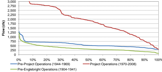
Exceedance Probability of Historical Mean Daily Yuba River Flow at Smartville Before and After Completion of Englebright Dam and the YRDP for September
