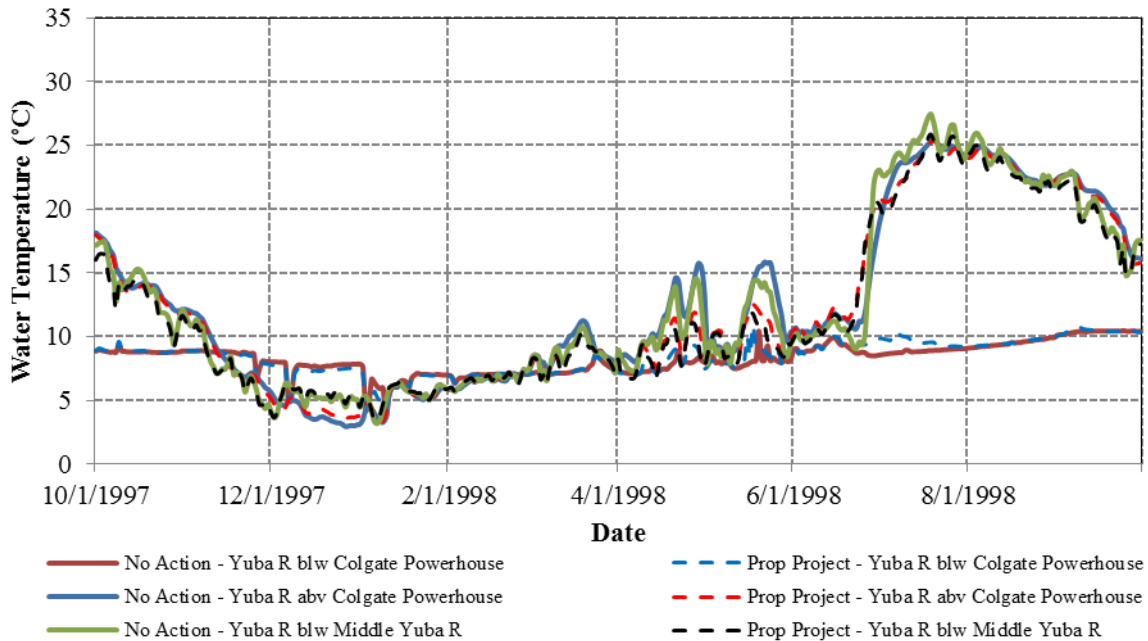
Figure 3.3.2-53. Simulated daily water temperatures for a representative wet WY (1998) at various locations along the Yuba River upstream of Englebright Reservoir.
