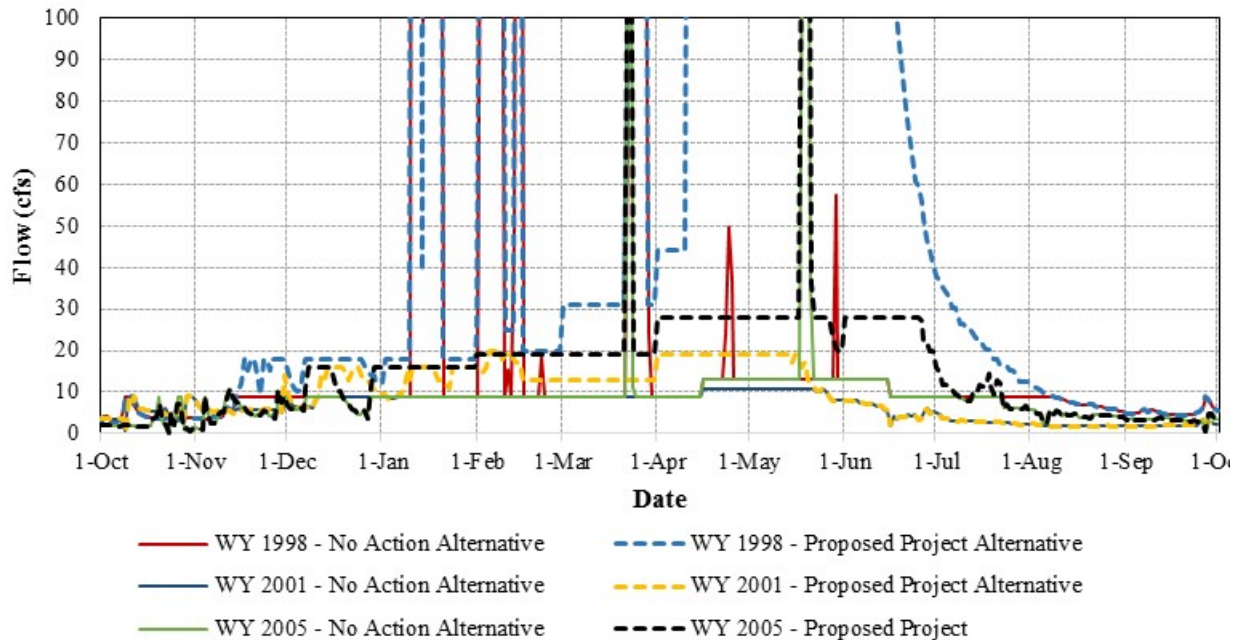
Figure 3.3.2-30. Simulated daily flows for Oregon Creek below Log Cabin Diversion Dam for the No Action and YCWA’s proposed Project for representative wet (1998), dry (2001) and normal (2005) WYs.
