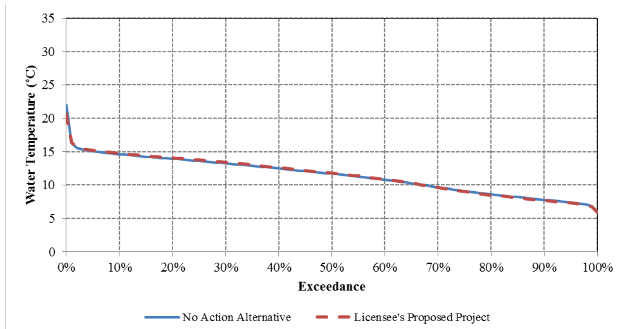
Figure 3.3.2-72. Exceedance curves of modeled mean daily water temperatures in the Yuba River downstream of Dry Creek for the No Action Alternative and Proposed Project Alternative for WYs 1970 through 2010.
