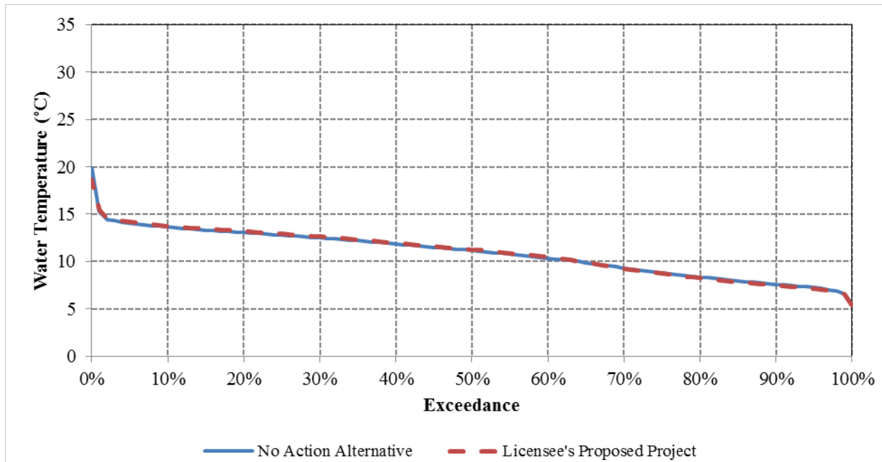
Figure 3.3.2-71. Exceedance curves of modeled mean daily water temperatures in the Yuba River near Parks Bar for the No Action Alternative and Proposed Project Alternative for WYs 1970 through 2010.
