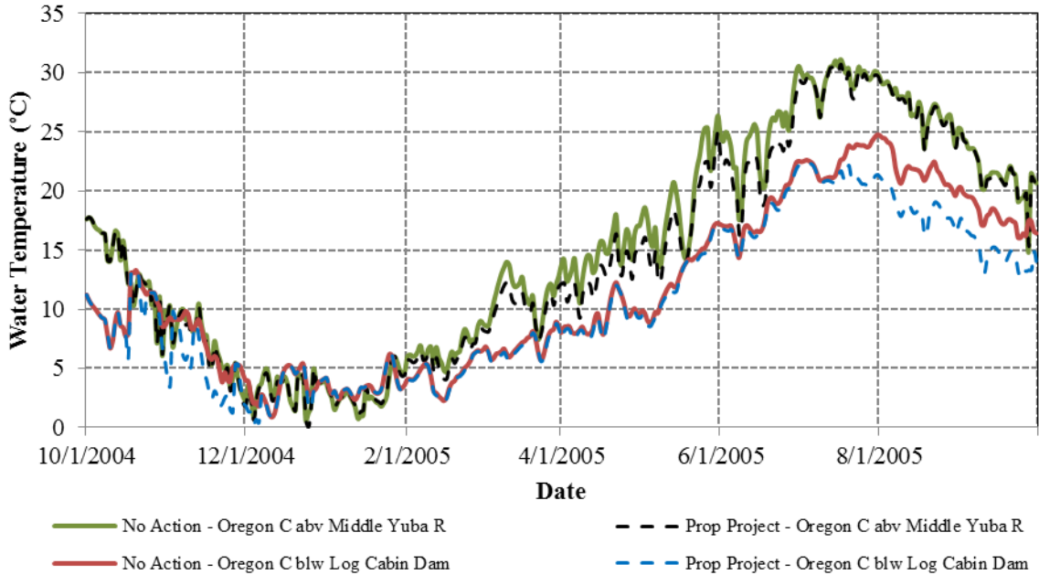
Figure 3.3.2-49. Simulated daily water temperatures for a representative normal WY (2005) at various locations along Oregon Creek.
