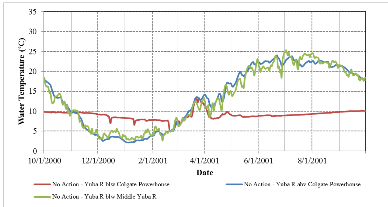
Figure 3.3.2-24. Simulated daily water temperatures for a representative dry WY (2001) at various locations along the Yuba River upstream of Englebright Reservoir.
