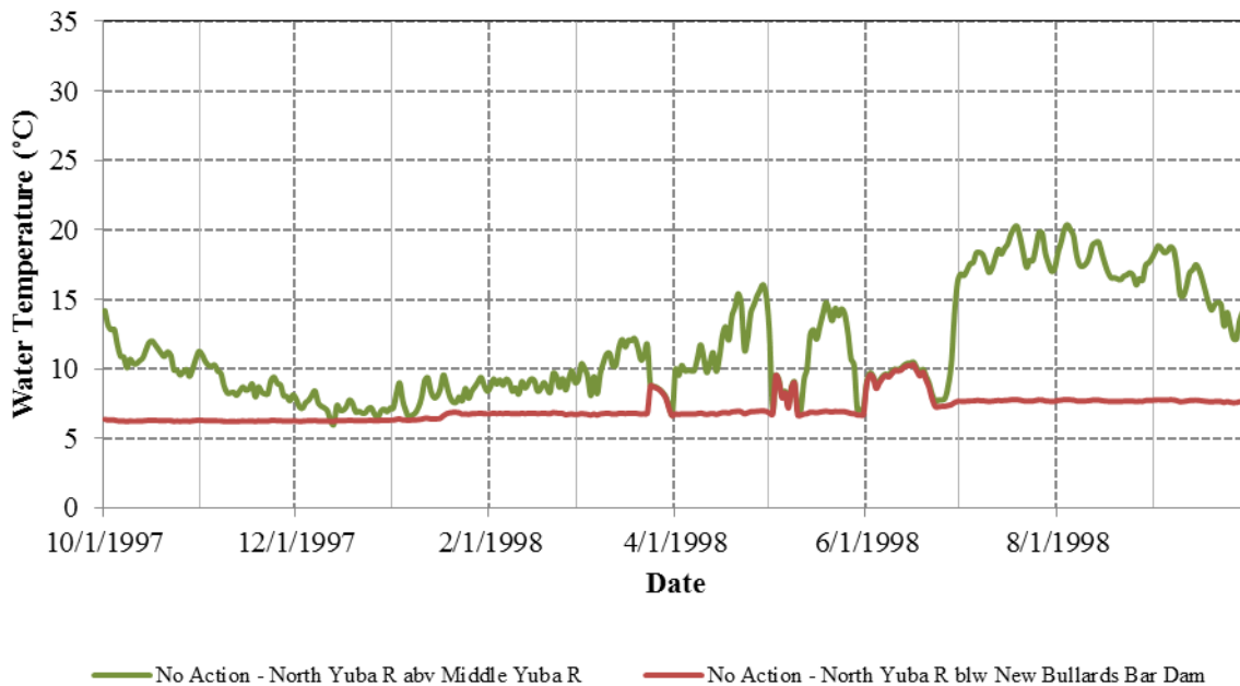
Figure 3.3.2-19. Simulated daily water temperatures for a representative wet WY (1998) at various locations along the North Yuba River.
