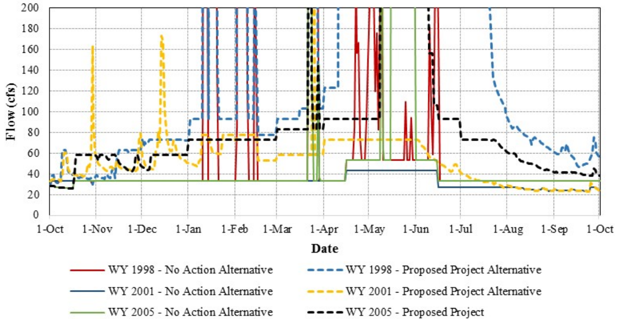
Figure 3.3.2-29. Simulated daily flows for the Middle Yuba River below Our House Diversion Dam for the No Action and YCWA’s proposed Project for representative wet (1998), dry (2001) and normal (2005) WYs.
