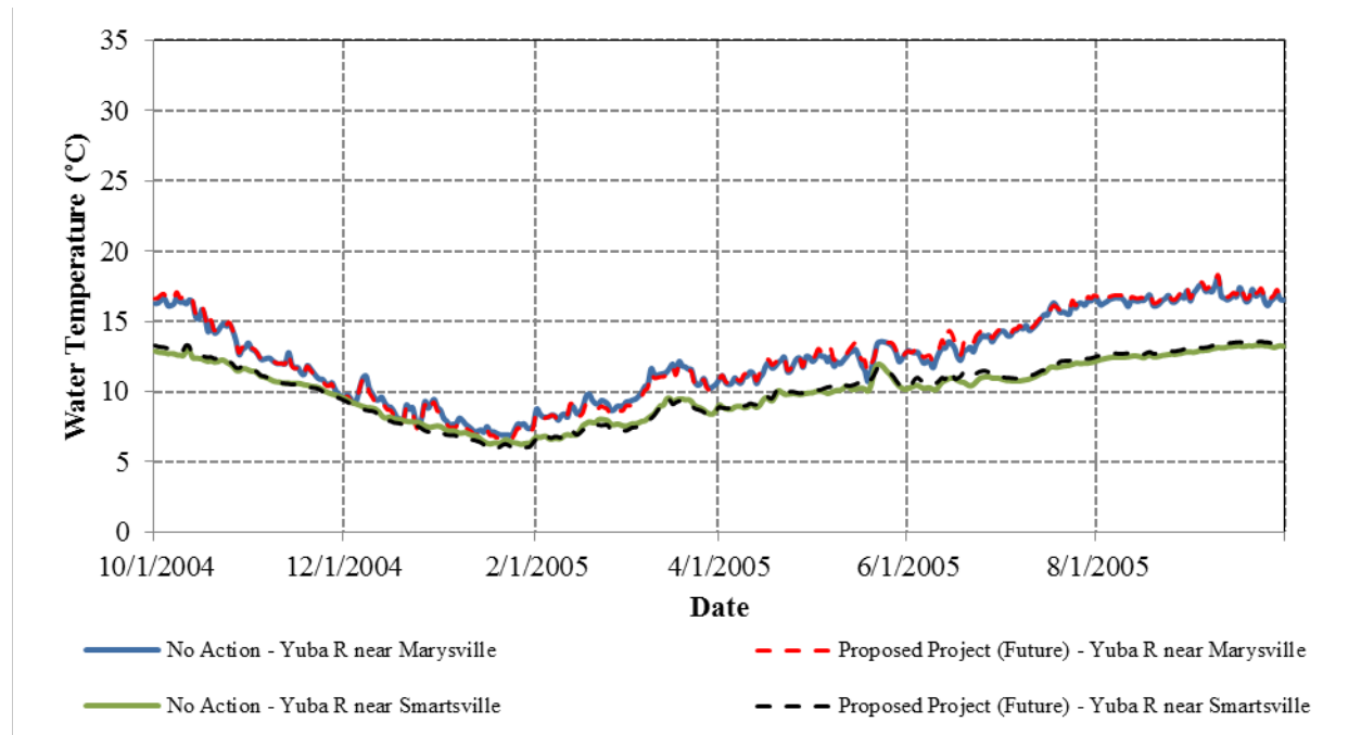
Figure 3.3.2-78. Simulated daily water temperatures for a representative normal WY (2005) at various locations along the Yuba River downstream of the Narrows 2 Powerhouse for the No Action Alternative compared to the Future Proposed Project Alternative.
