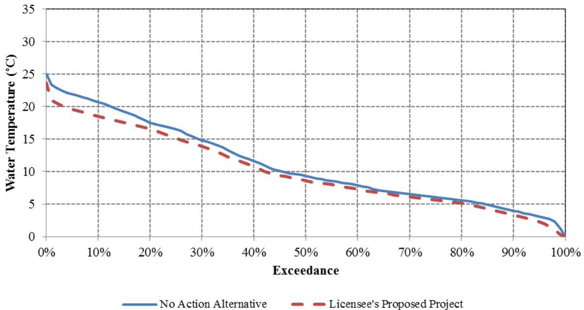
Figure 3.3.2-63. Exceedance curves of modeled mean daily water temperatures in Oregon Creek downstream of Log Cabin Diversion Dam for the No Action Alternative and Proposed Project Alternative for WYs 1970 through 2010.
