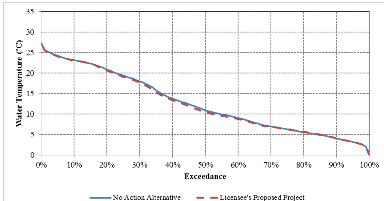
Figure 3.3.2-60. Exceedance curves of modeled mean daily water temperatures in the Middle Yuba River upstream of Oregon Creek for the No Action Alternative and Proposed Project Alternative for WYs 1970 through 2010.
