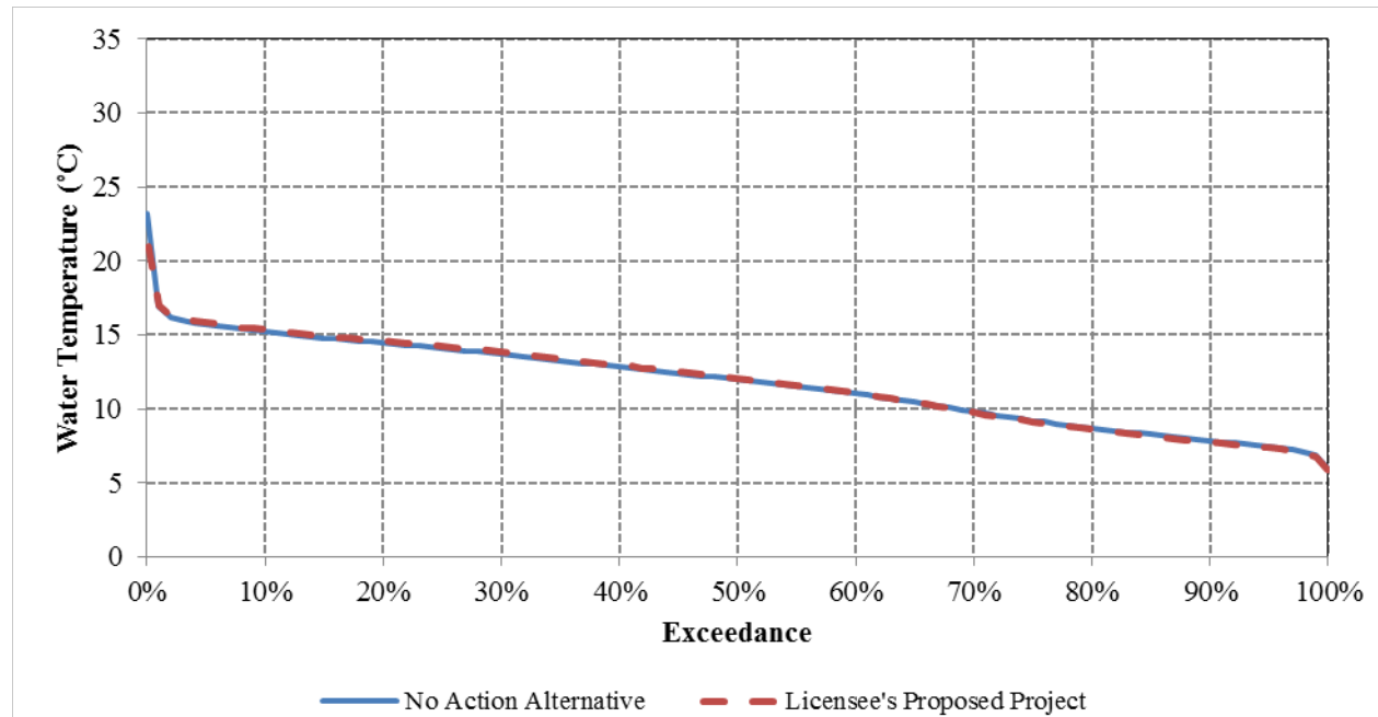
Figure 3.3.2-73. Exceedance curves of modeled mean daily water temperatures in the Yuba River downstream of Daguerre Point Dam for the No Action Alternative and Proposed Project Alternative for WYs 1970 through 2010.
