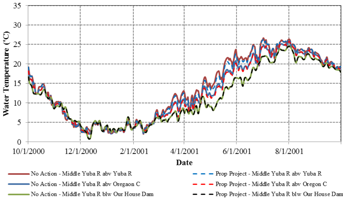
Figure 3.3.2-45. Simulated daily water temperatures for a representative dry WY (2001) at various locations along the Middle Yuba River.
