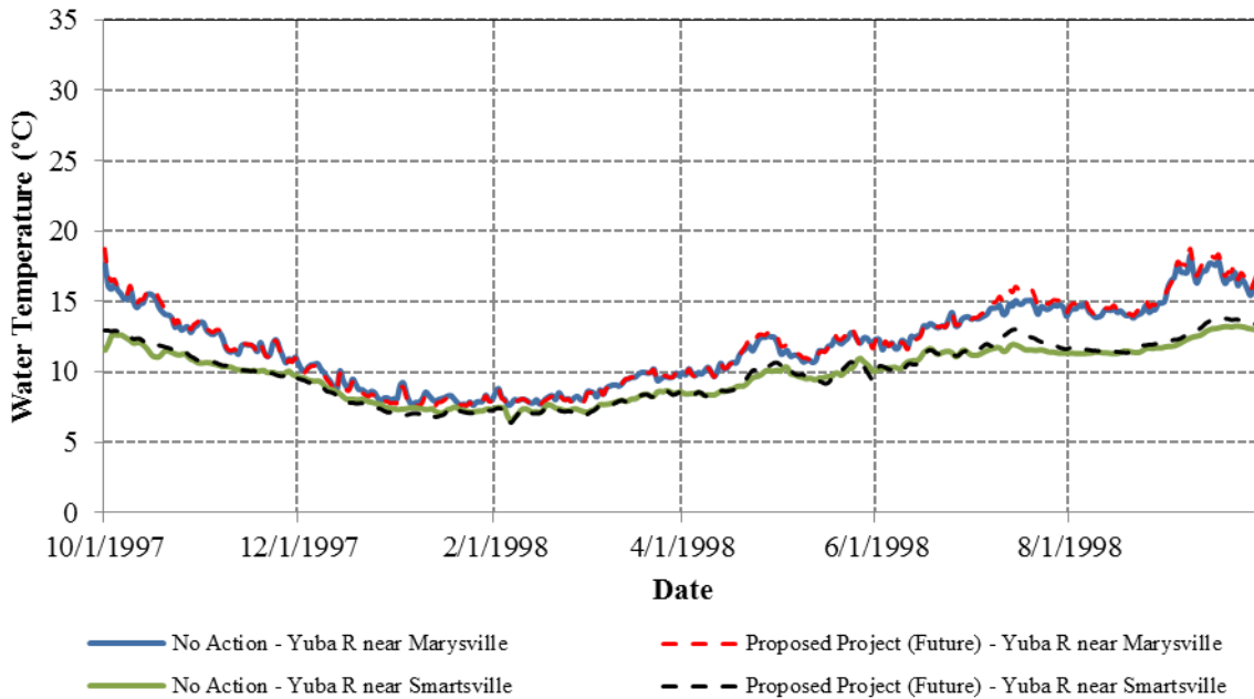
Figure 3.3.2-76. Simulated daily water temperatures for a representative wet WY (1998) at various locations along the Yuba River downstream of the Narrows 2 Powerhouse for the No Action Alternative compared to the Future Proposed Project Alternative.
