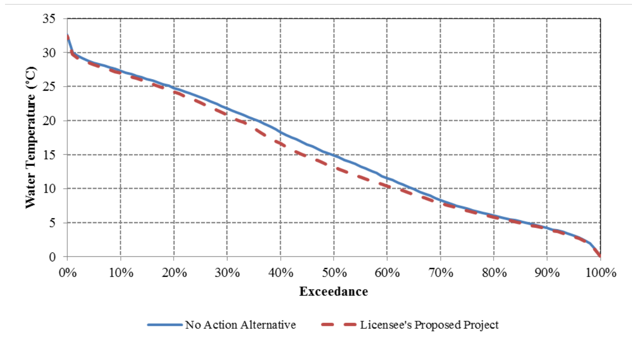
Figure 3.3.2-64. Exceedance curves of modeled mean daily water temperatures in Oregon Creek upstream of the Middle Yuba River for the No Action Alternative and Proposed Project Alternative for WYs 1970 through 2010.
