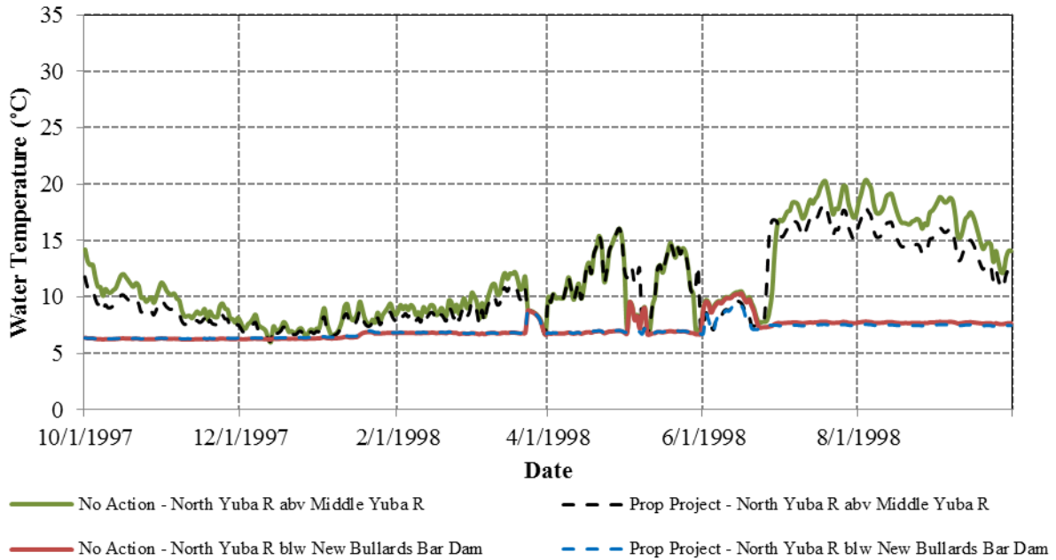
Figure 3.3.2-50. Simulated daily water temperatures for a representative wet WY (1998) at various locations along the North Yuba River.
