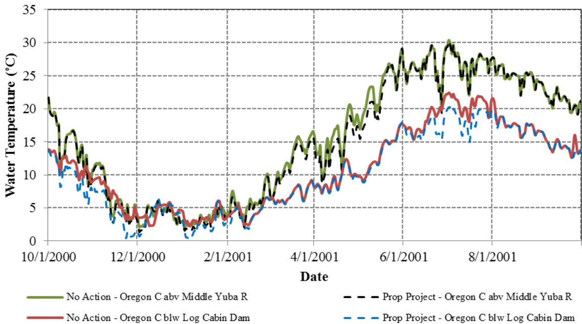
Figure 3.3.2-48. Simulated daily water temperatures for a representative dry WY (2001) at various locations along Oregon Creek.
