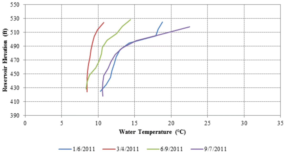
Figure 3.3.2-8. Englebright Reservoir water temperature profiles at four dates in 2011.
