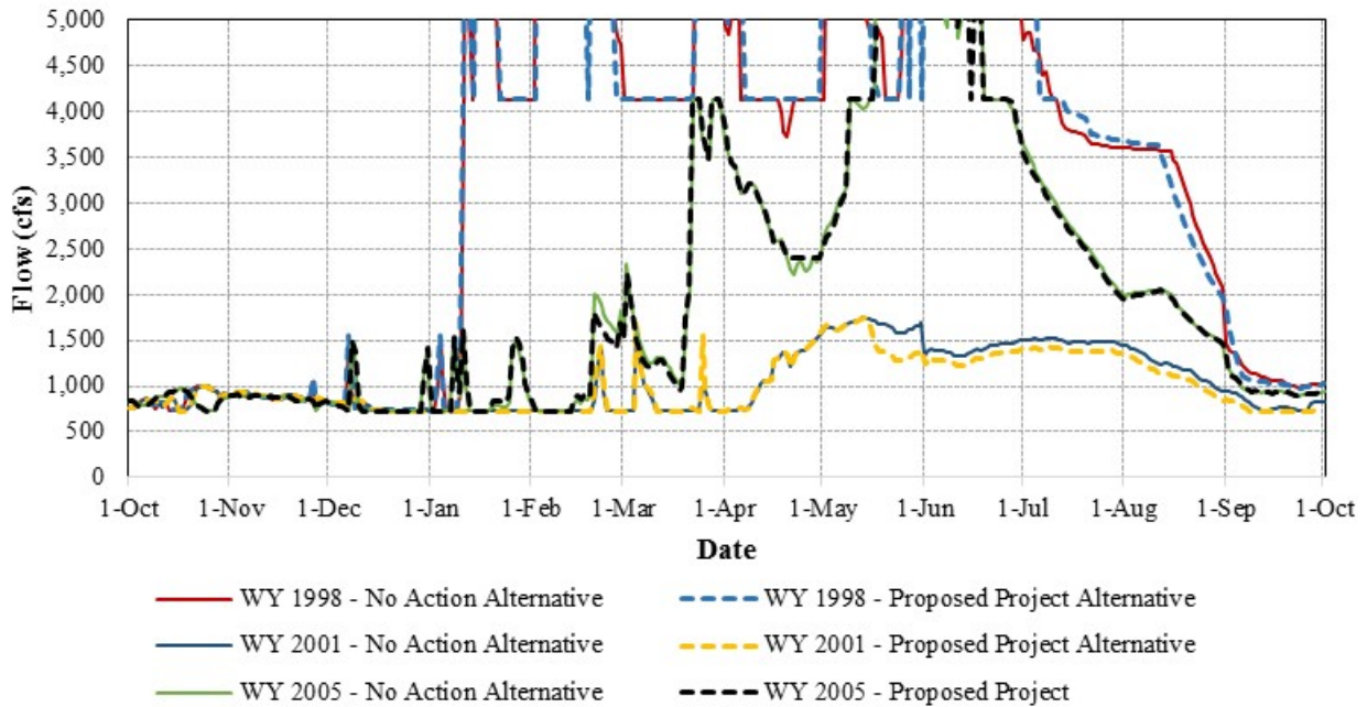
Figure 3.3.2-32. Simulated daily flows for the Yuba River near Smartsville for the No Action and YCWA’s proposed Project for representative wet (1998), dry (2001) and normal (2005) WYs.
