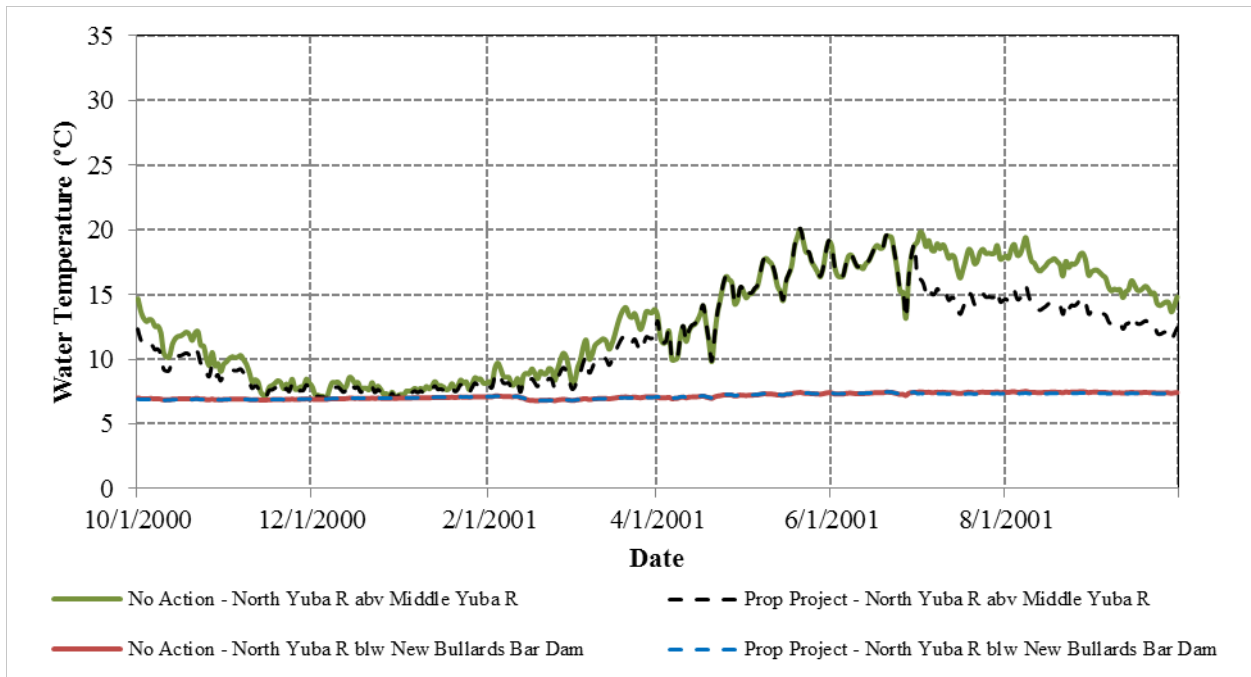
Figure 3.3.2-51. Simulated daily water temperatures for a representative dry WY (2001) at various locations along the North Yuba River.
