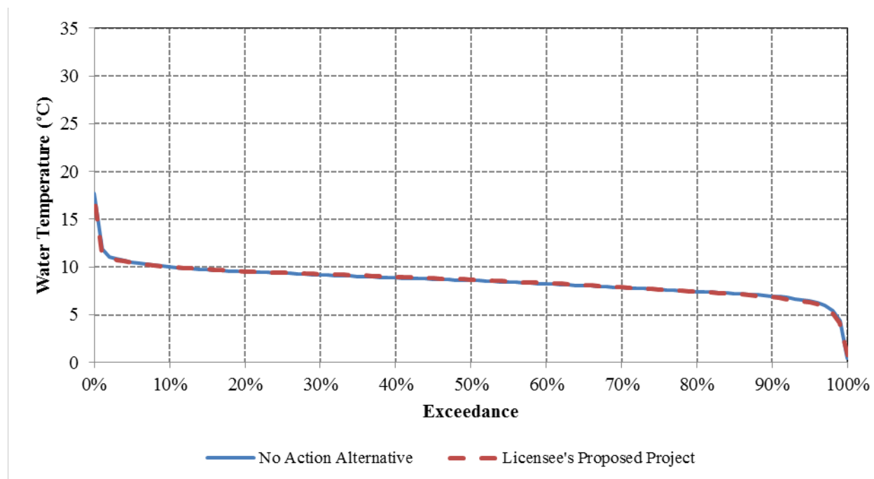
Figure 3.3.2-68. Exceedance curves of modeled mean daily water temperatures in the Yuba River downstream of the New Colgate Powerhouse for the No Action Alternative and Proposed Project Alternative for WYs 1970 through 2010.
