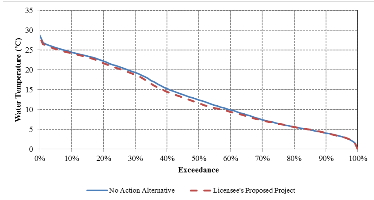
Figure 3.3.2-62. Exceedance curves of modeled mean daily water temperatures in the Middle Yuba River upstream of the North Yuba River for the No Action Alternative and Proposed Project Alternative for WYs 1970 through 2010.
