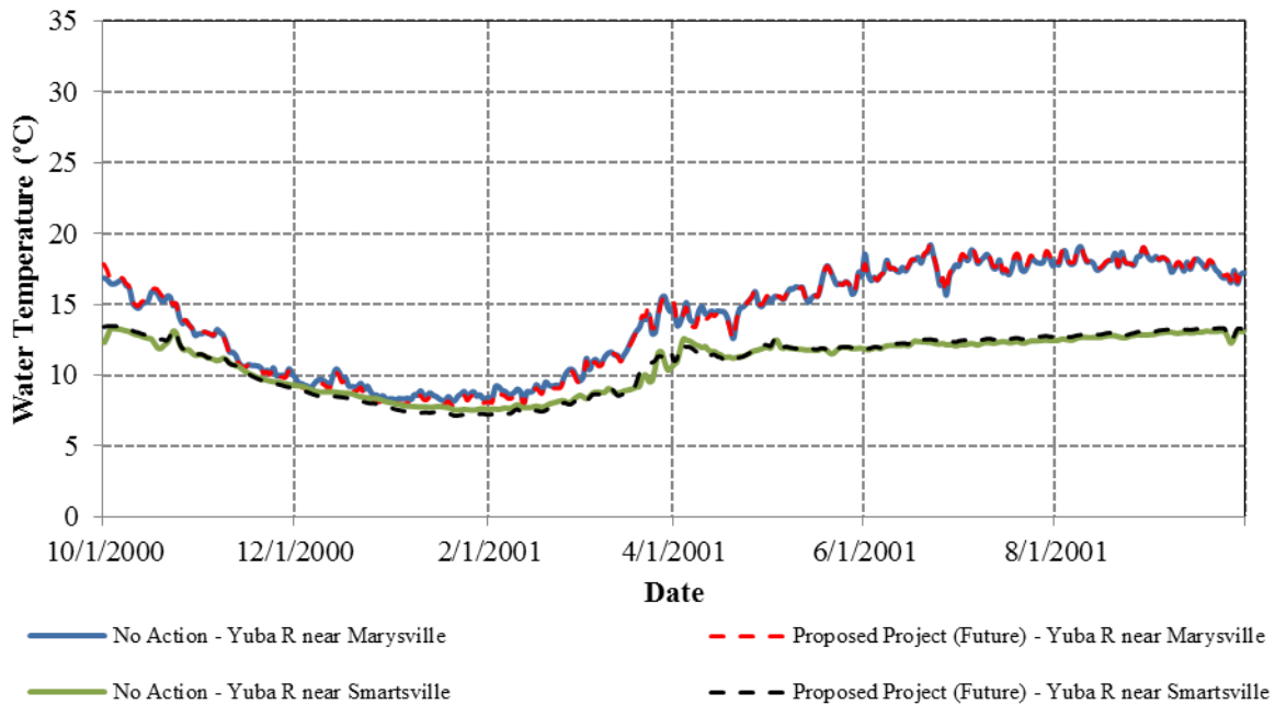
Figure 3.3.2-77. Simulated daily water temperatures for a representative dry WY (2001) at various locations along the Yuba River downstream of the Narrows 2 Powerhouse for the No Action Alternative compared to the Future Proposed Project Alternative.
