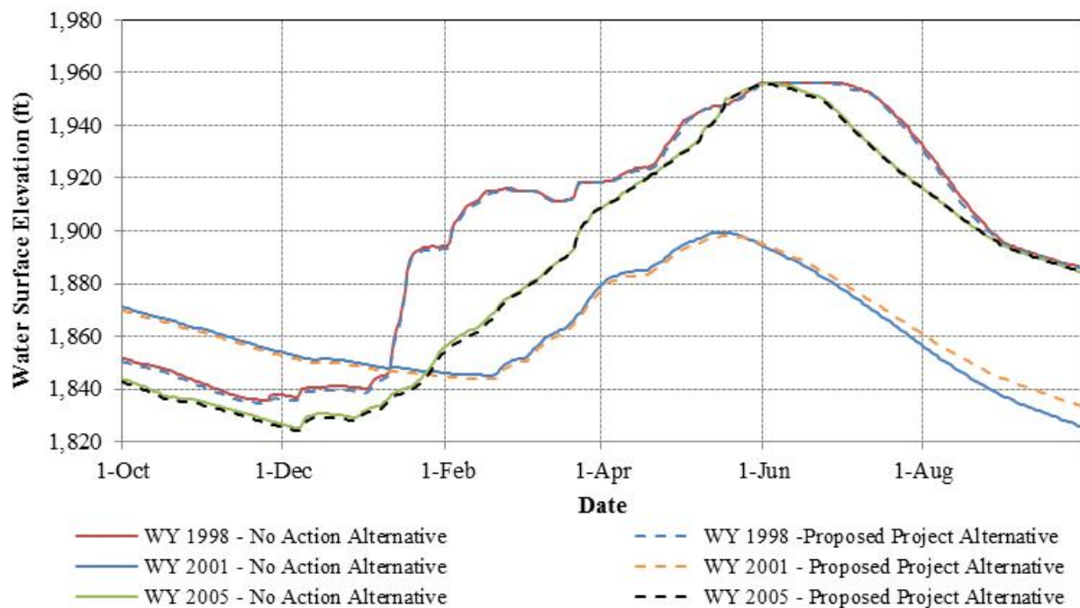
Figure 3.3.2-33. Simulated daily New Bullards Bar Reservoir water surface elevation for the No Action and YCWA’s proposed Project for representative wet (1998), dry (2001) and normal (2005) WYs.
