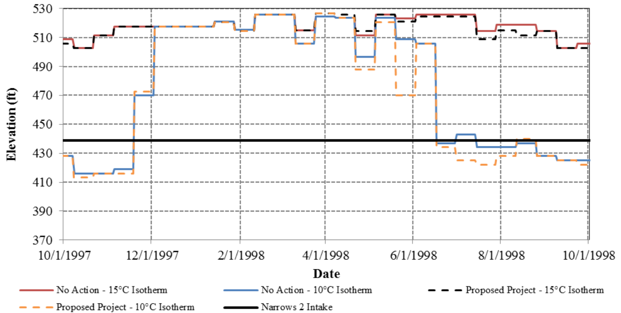
Figure 3.3.2-39. Simulated bi-weekly Englebright Reservoir 10°C and 15°C isotherm elevations for the No Action and YCWA’s proposed Project for a representative wet (1998) WY. The elevation of the Narrows 2 Power Tunnel intake is shown.
