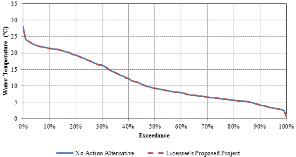
Figure 3.3.2-59. Exceedance curves of modeled mean daily water temperatures in the Middle Yuba River downstream of Our House Dam for the No Action Alternative and Proposed Project Alternative for WYs 1970 through 2010.
