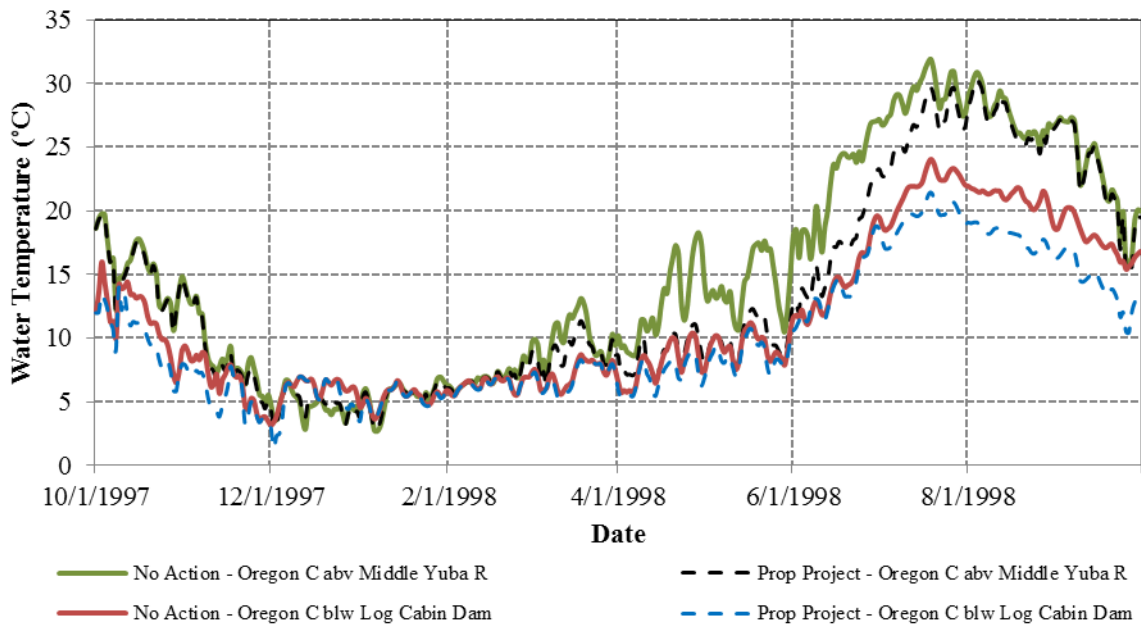
Figure 3.3.2-47. Simulated daily water temperatures for a representative wet WY (1998) at various locations along Oregon Creek.
