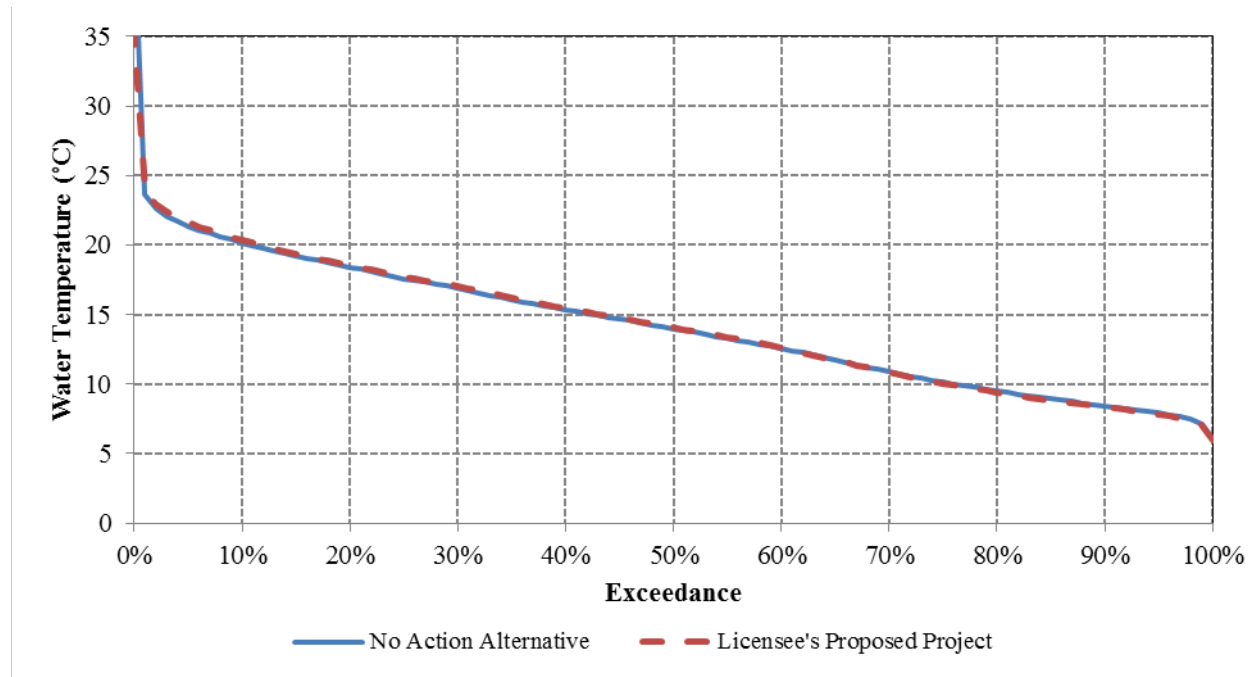
Figure 3.3.2-75. Exceedance curves of modeled mean daily water temperatures in the Yuba River upstream of the Feather River for the No Action Alternative and Proposed Project Alternative for WYs 1970 through 2010.
