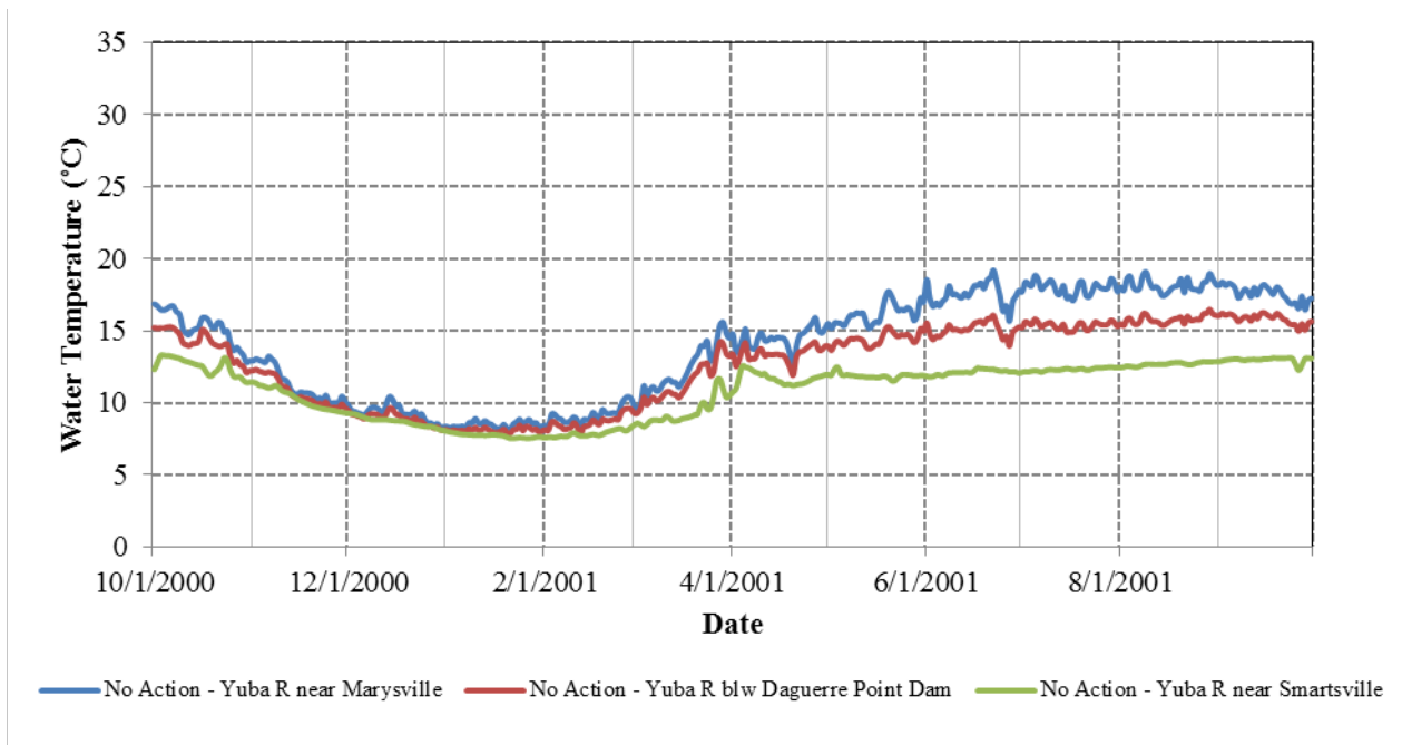
Figure 3.3.2-27. Simulated daily water temperatures for a representative dry WY (2001) at various locations along the Yuba River downstream of the Narrows 2 Powerhouse.
