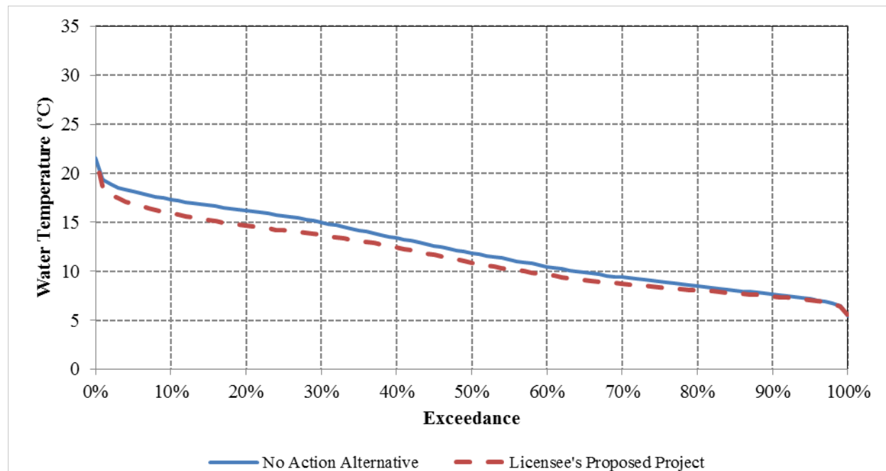
Figure 3.3.2-65. Exceedance curves of modeled mean daily water temperatures in the North Yuba River upstream of the Middle Yuba River for the No Action Alternative and Proposed Project Alternative for WYs 1970 through 2010.
