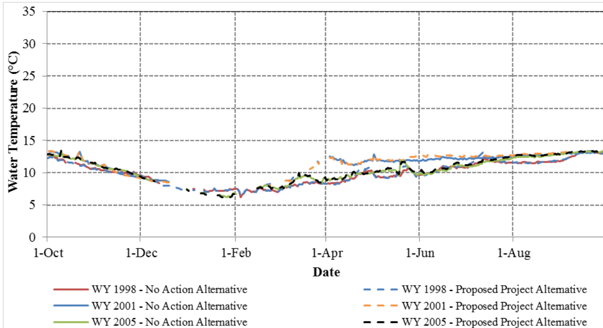
Figure 3.3.2-42. Simulated daily Narrows 2 Powerhouse release water temperatures for representative wet (1998), dry (2001), and normal (2005) water years.
