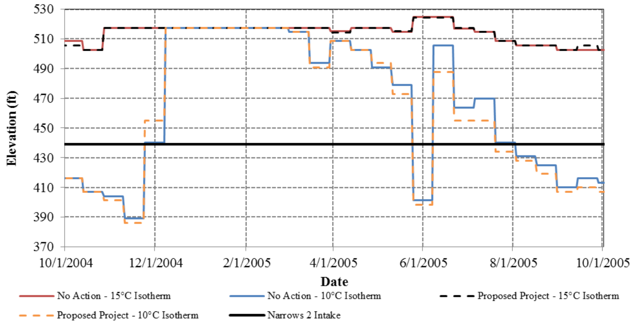
Figure 3.3.2-41. Simulated bi-weekly Englebright Reservoir 10°C and 15°C isotherm elevations for the No Action and YCWA’s proposed Project for a representative normal (2005) WY. The elevation of the Narrows 2 Power Tunnel intake is shown.
