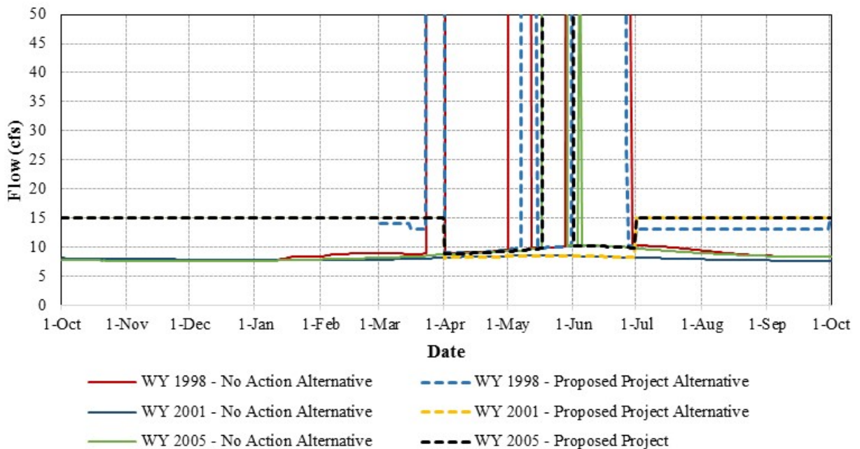
Figure 3.3.2-31. Simulated daily flows for the North Yuba River below New Bullards Bar Reservoir for the No Action and YCWA’s proposed Project for representative wet (1998), dry (2001) and normal (2005) WYs.
