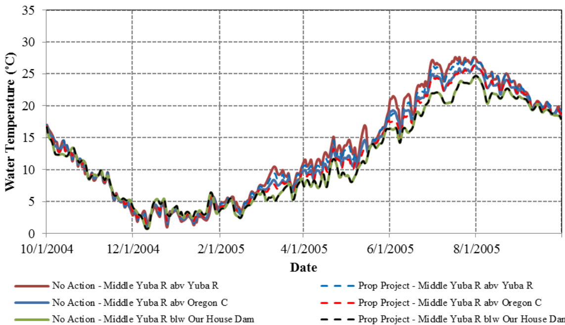
Figure 3.3.2-46. Simulated daily water temperatures for a representative normal WY (2005) at various locations along the Middle Yuba River
