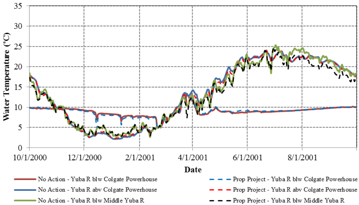
Figure 3.3.2-54. Simulated daily water temperatures for a representative dry WY (2001) at various locations along the Yuba River upstream of Englebright Reservoir.
