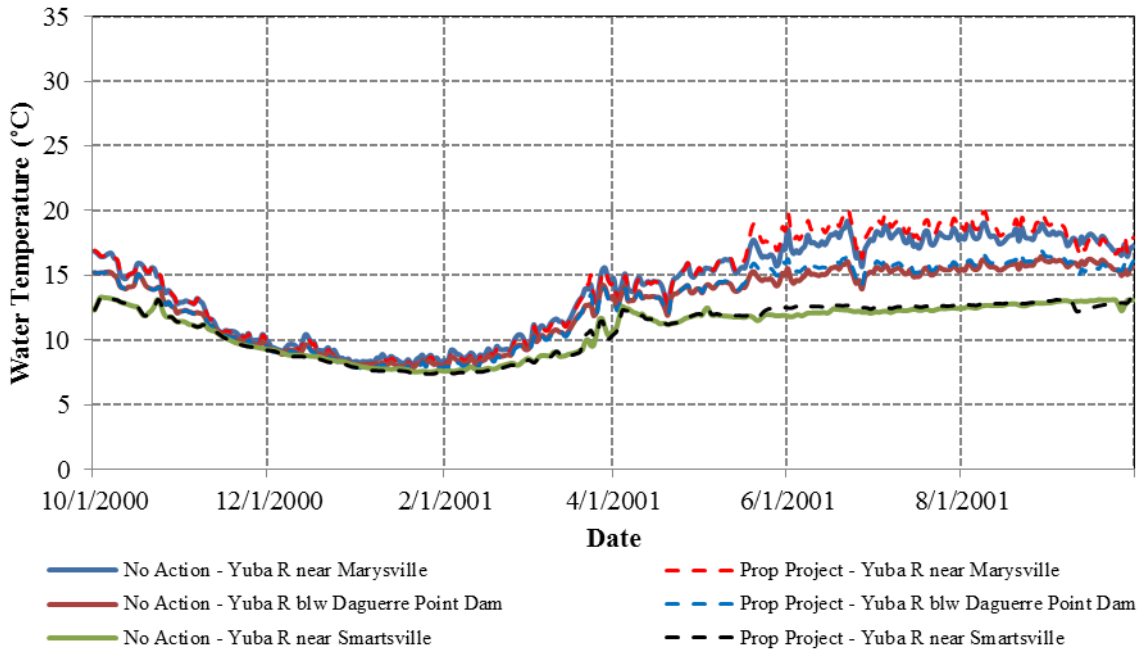
Figure 3.3.2-57. Simulated daily water temperatures for a representative dry WY (2001) at various locations along the Yuba River downstream of the Narrows 2 Powerhouse.
