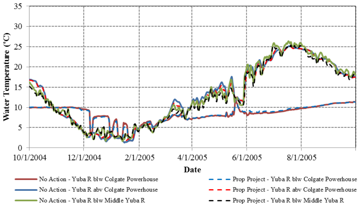
Figure 3.3.2-55. Simulated daily water temperatures for a representative normal WY (2005) at various locations along the Yuba River upstream of Englebright Reservoir.
