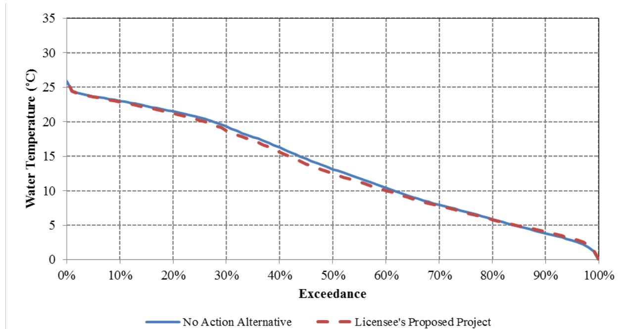
Figure 3.3.2-67. Exceedance curves of modeled mean daily water temperatures in the Yuba River upstream of the New Colgate Powerhouse for the No Action Alternative and Proposed Project Alternative for WYs 1970 through 2010.
