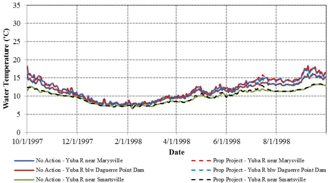
Figure 3.3.2-56. Simulated daily water temperatures for a representative wet WY (1998) at various locations along the Yuba River downstream of the Narrows 2 Powerhouse.
