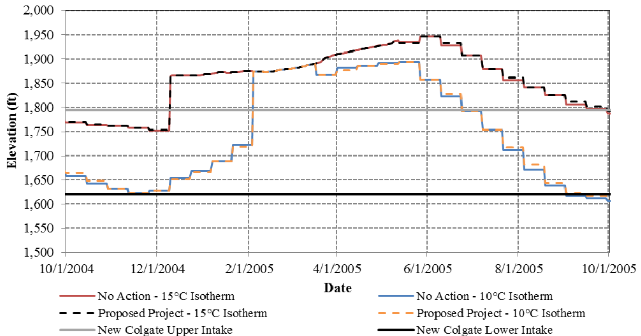
Figure 3.3.2-36. Simulated bi-weekly New Bullards Bar Reservoir 10°C and 15°C isotherm elevations for the No Action and YCWA’s proposed Project for a representative normal (2005) WY. The elevation of the New Colgate Power Tunnel upper and lower intakes is shown.
