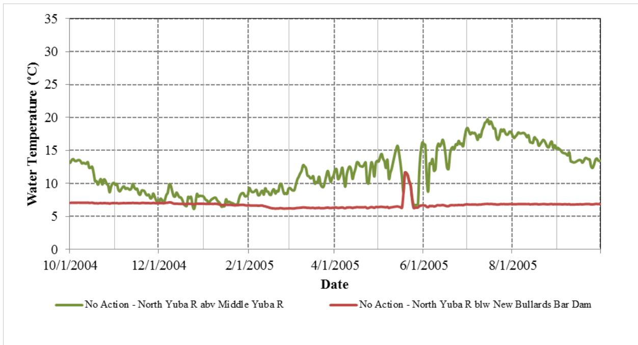
Figure 3.3.2-21. Simulated daily water temperatures for a representative normal WY (2005) at various locations along the North Yuba River.
