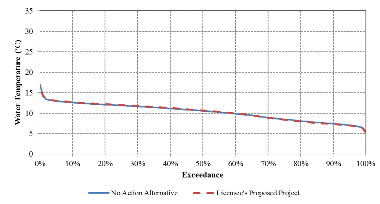
Figure 3.3.2-69. Exceedance curves of modeled mean daily water temperatures in the Yuba River near Smartsville for the No Action Alternative and Proposed Project Alternative for WYs 1970 through 2010.
