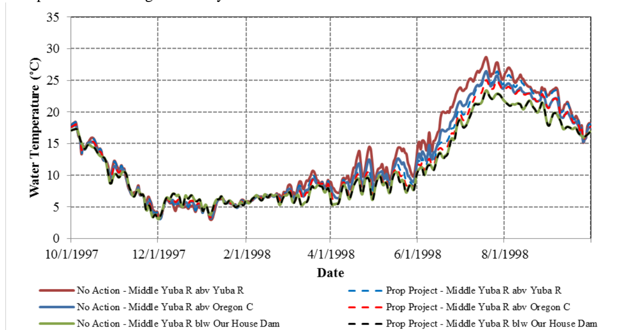
Figure 3.3.2-44. Simulated daily water temperatures for a representative wet WY (1998) at various locations along the Middle Yuba River.
