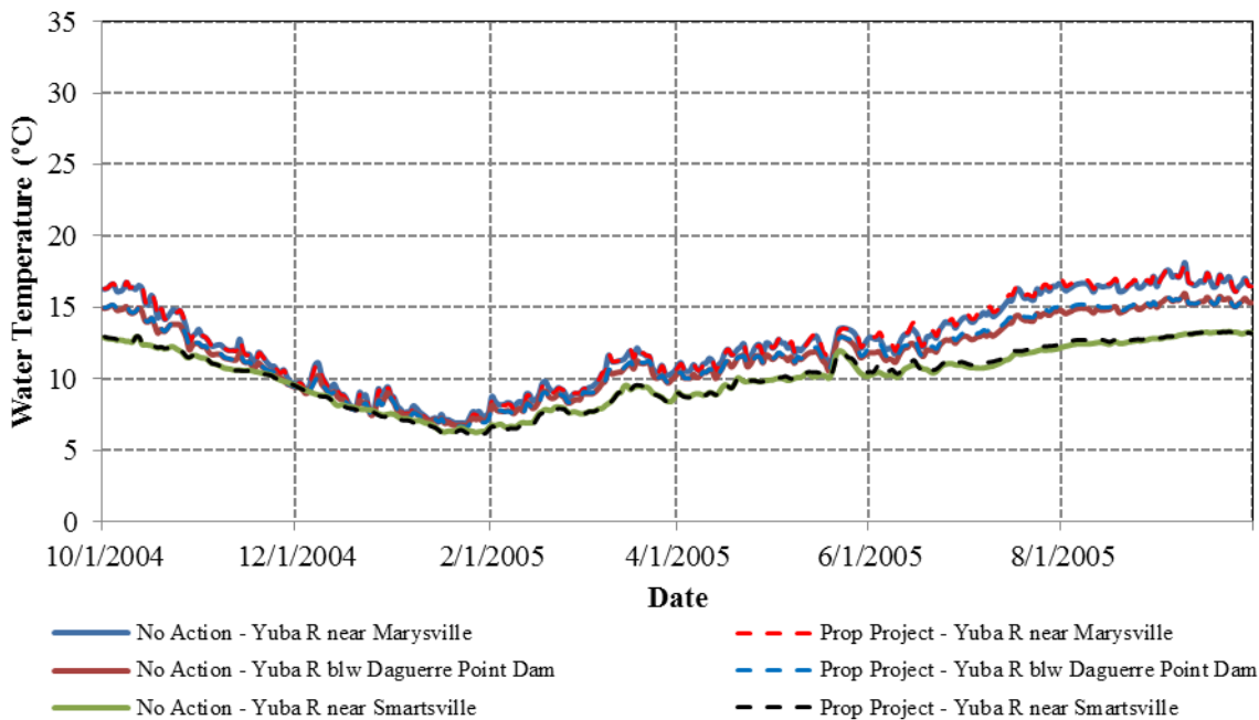
Figure 3.3.2-58. Simulated daily water temperatures for a representative normal WY (2005) at various locations along the Yuba River downstream of the Narrows 2 Powerhouse.
