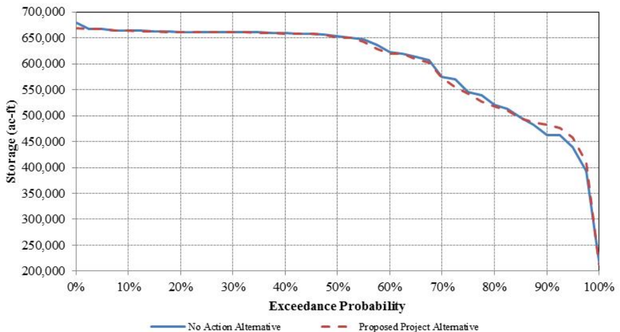
Figure 3.3.2-37. Simulated exceedance probability of end-of-September New Bullards Bar Reservoir storage for the No Action and YCWA’s proposed Project for WYs 1970 through 2010.
