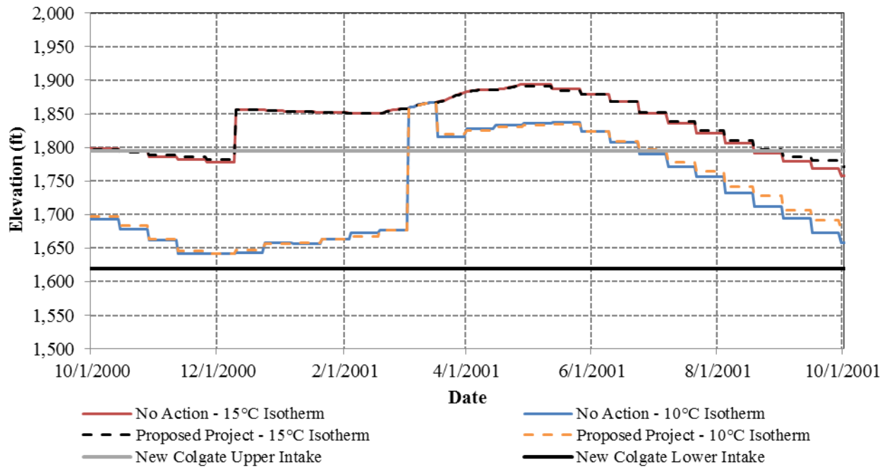
Figure 3.3.2-35. Simulated bi-weekly New Bullards Bar Reservoir 10°C and 15°C isotherm elevations for the No Action and YCWA’s proposed Project for a representative dry (2001) WY. The elevation of the New Colgate Power Tunnel upper and lower intakes is shown.
