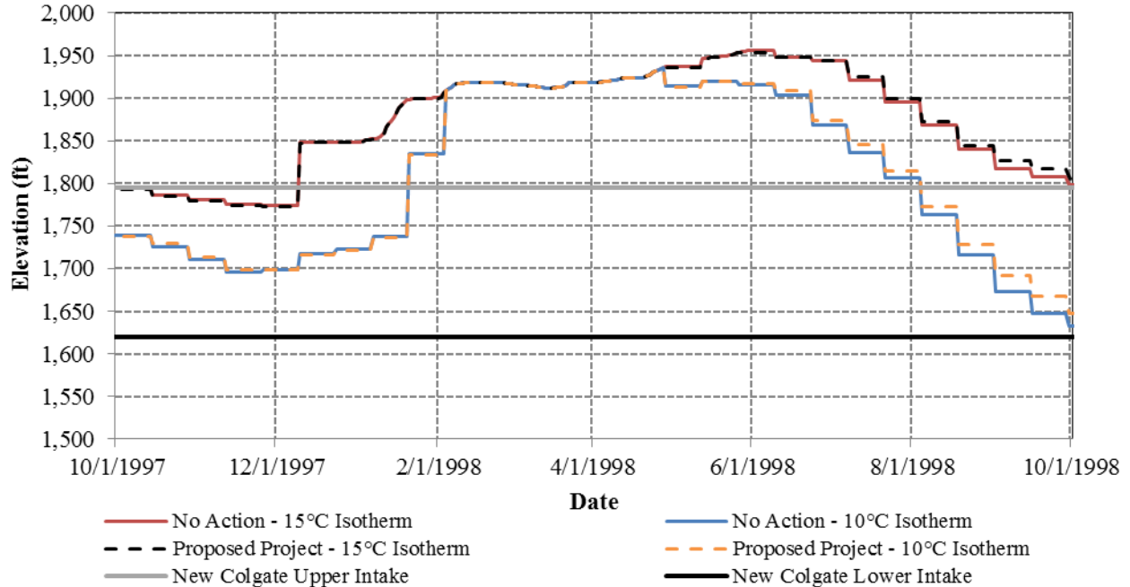
Figure 3.3.2-34. Simulated bi-weekly New Bullards Bar Reservoir 10°C and 15°C isotherm elevations for the No Action and YCWA’s proposed Project for a representative wet (1998) WY. The elevation of the New Colgate Power Tunnel and lower intakes is shown.
