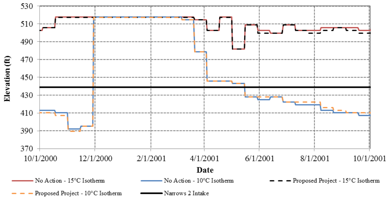
Figure 3.3.2-40. Simulated bi-weekly Englebright Reservoir 10°C and 15°C isotherm elevations for the No Action and YCWA’s proposed Project for a representative dry (2001) WY. The elevation of the Narrows 2 Power Tunnel intake is shown.
