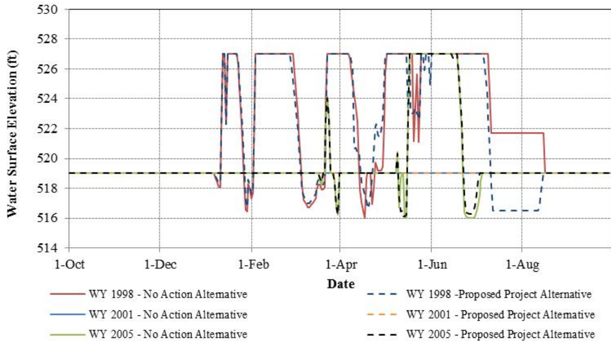
Figure 3.3.2-38. Simulated daily Englebright Reservoir water surface elevation for the No Action and YCWA’s proposed Project for representative wet (1998), dry (2001) and normal (2005) WYs.
