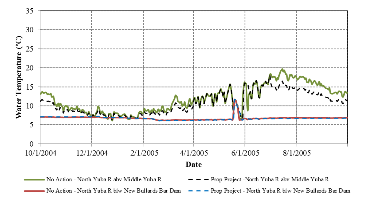
Figure 3.3.2-52. Simulated daily water temperatures for a representative dry WY (2005) at various locations along the North Yuba River.
