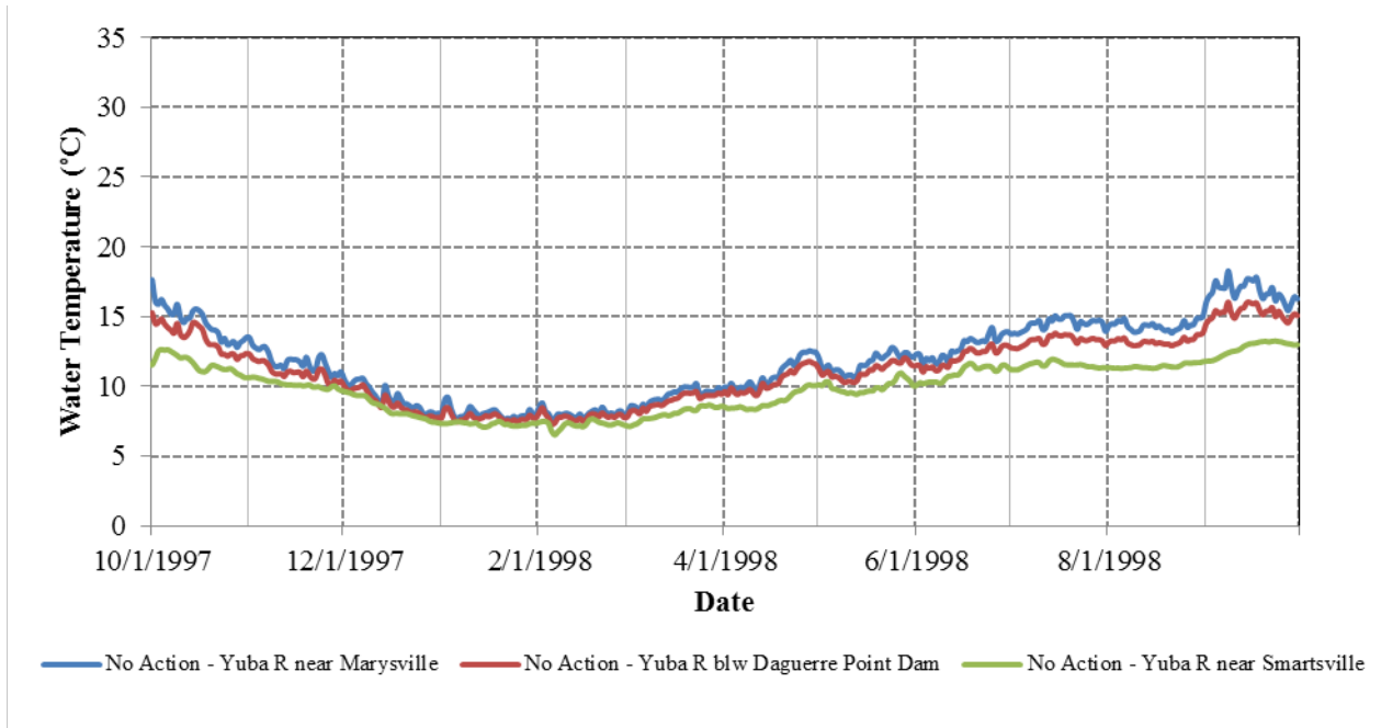
Figure 3.3.2-26. Simulated daily water temperatures for a representative wet WY (1998) at various locations along the Yuba River downstream of the Narrows 2 Powerhouse.
