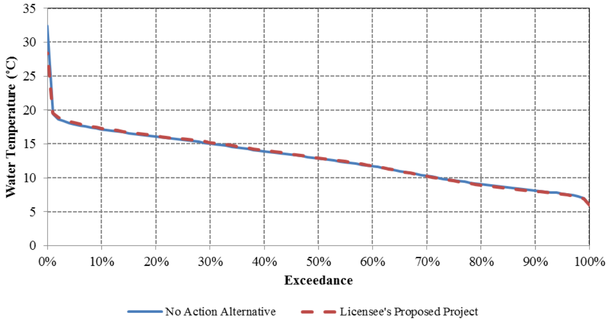
Figure 3.3.2-74. Exceedance curves of modeled mean daily water temperatures in the Yuba River near Marysville for the No Action Alternative and Proposed Project Alternative for WYs 1970 through 2010.
