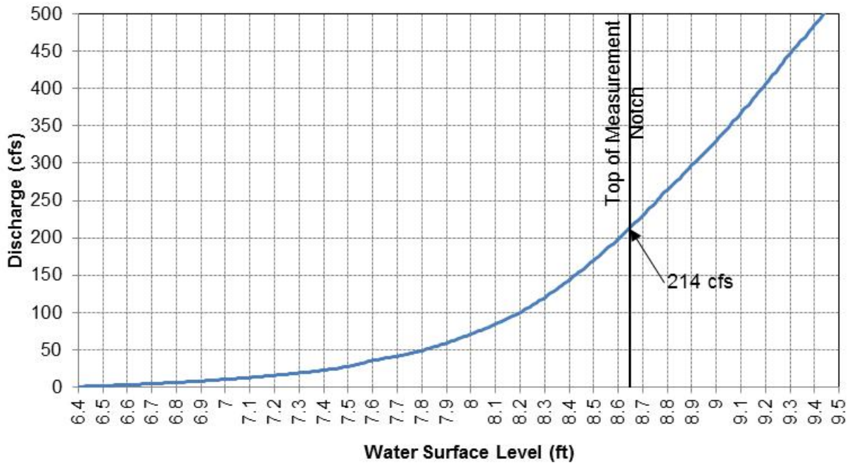
Figure 5.1-2. Existing ratings curve for the Oregon Creek below Log Cabin Diversion Dam measurement weir and its current measurement notch capacity.
