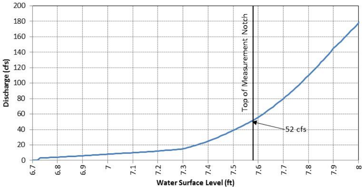
Figure 5.1-3. Existing ratings curve for the North Yuba River below New Bullards Bar Dam measurement weir and its current measurement notch capacity.
