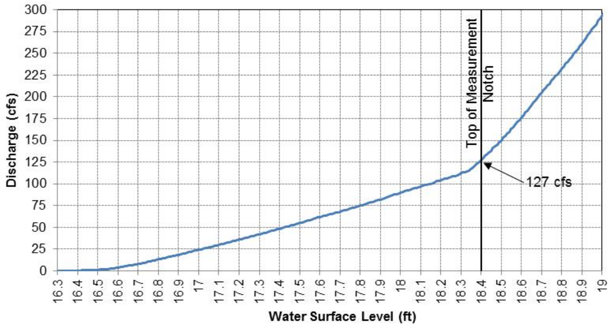
Figure 5.1-1. Existing ratings curve for the Middle Yuba River below Our House Diversion Dam measurement weir and its current measurement notch capacity.
