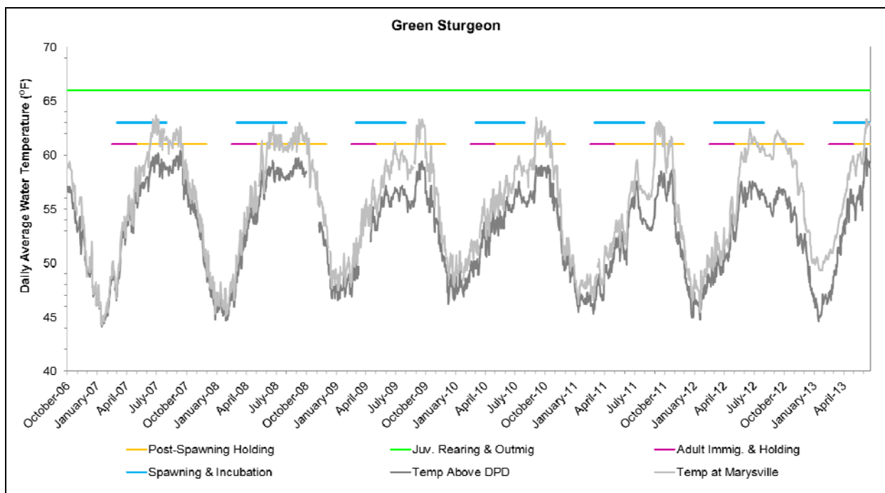
Figure 4. Lower Yuba River monitored water temperatures and green sturgeon upper tolerance water temperature index values.
