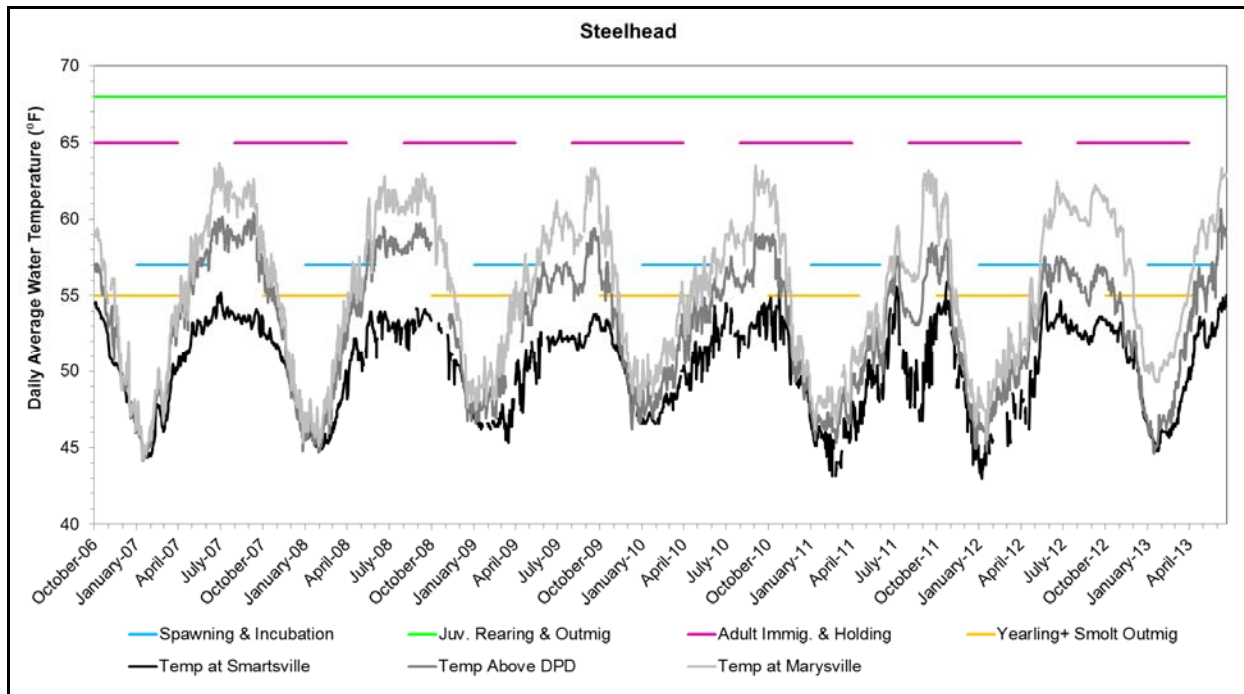
Figure 3.1-1. Lower Yuba River monitored water temperatures and steelhead upper tolerance water temperature index values.
