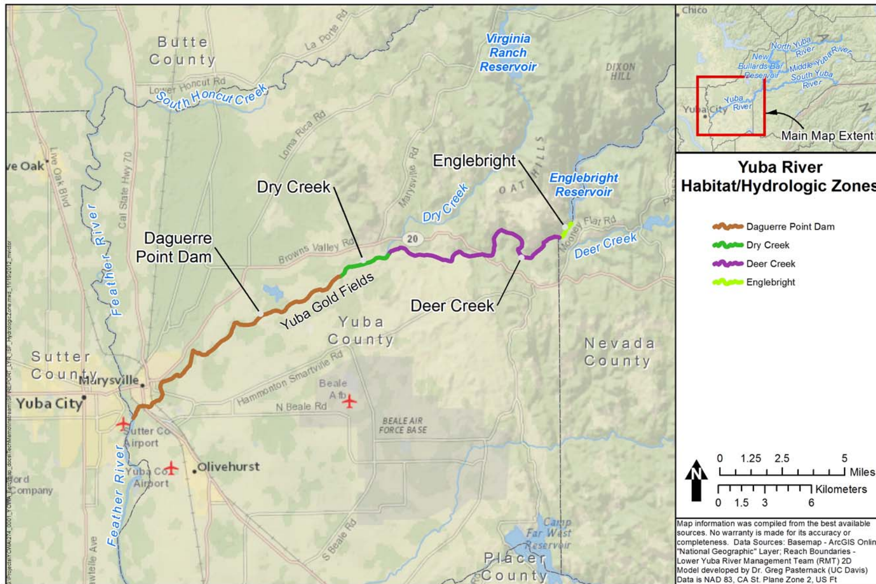
Figure 2.1-1. Hydrologic reaches in the Yuba River downstream of Englebright Dam.
