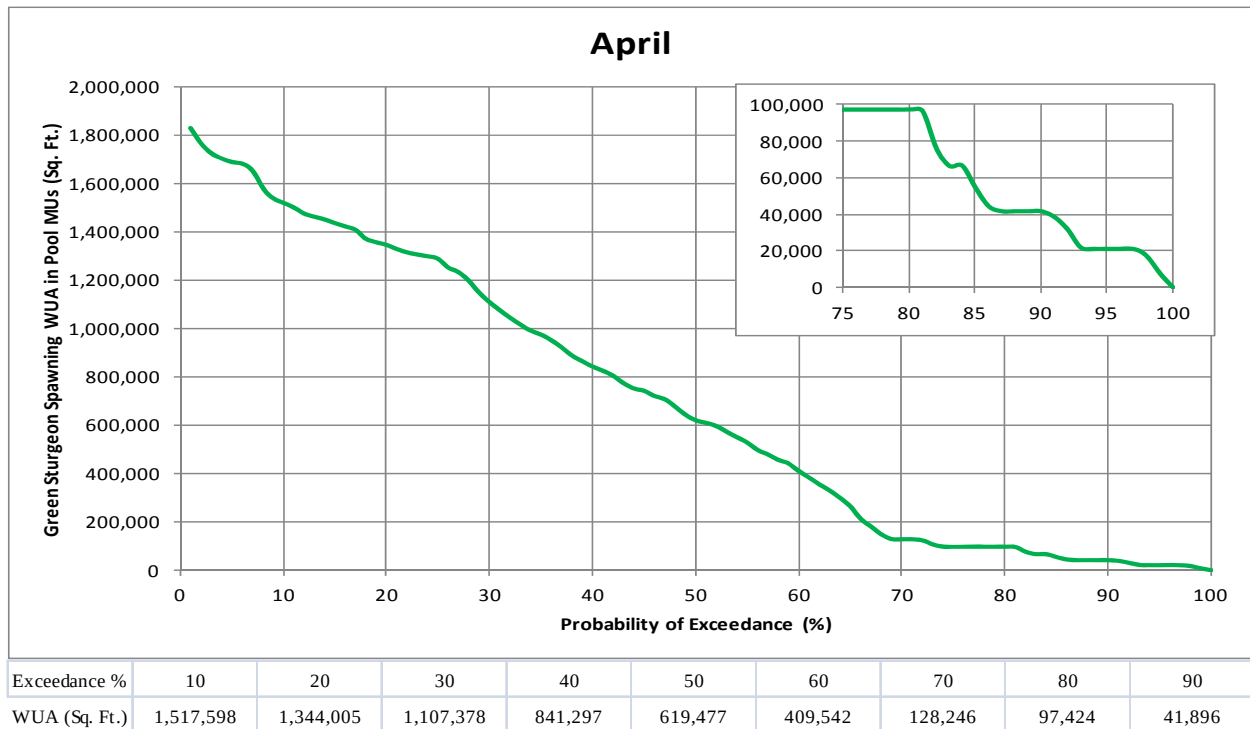
Figure 3.4-16. Simulated green sturgeon spawning WUA exceedance (in pool morphological units) during April for WY 1970 through 2010.
