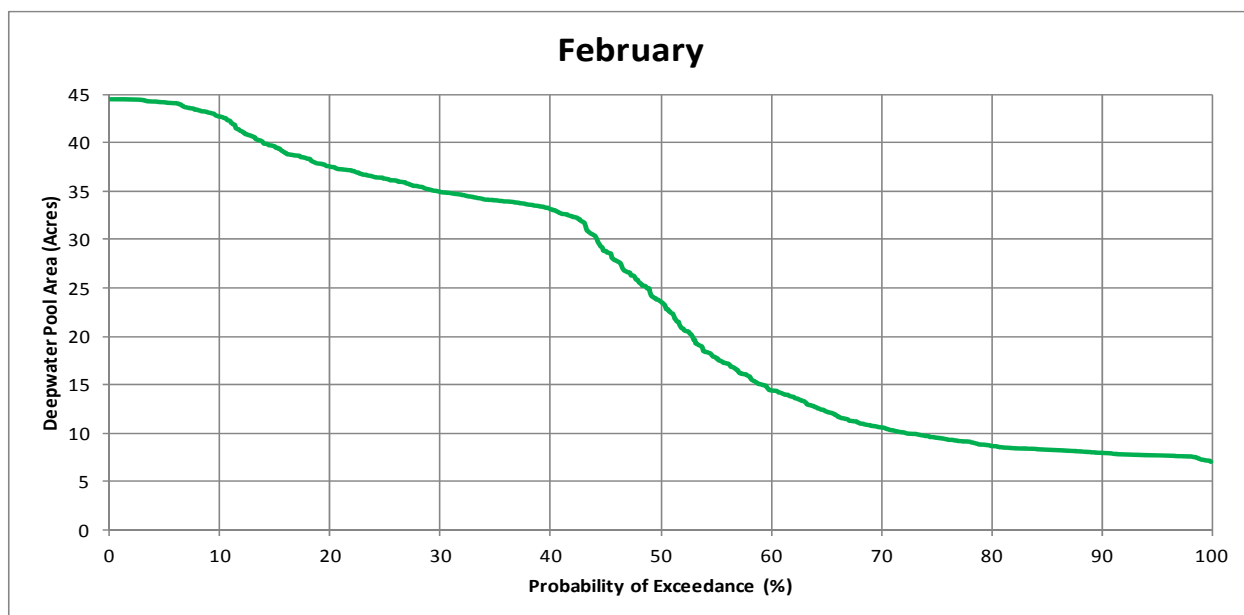
Figure 3.4-2. Simulated adult green sturgeon deepwater holding habitat exceedance during February for WY 1970 through 2010.
