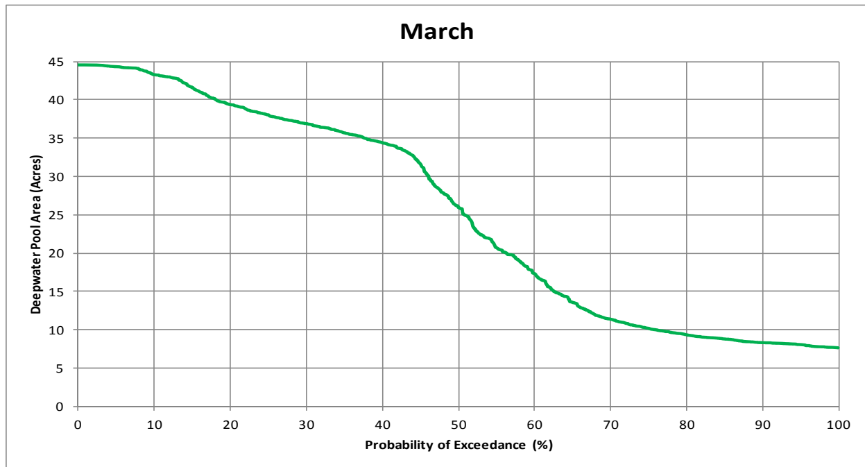
Figure 3.4-3. Simulated adult green sturgeon deepwater holding habitat exceedance during March for WY 1970 through 2010.
