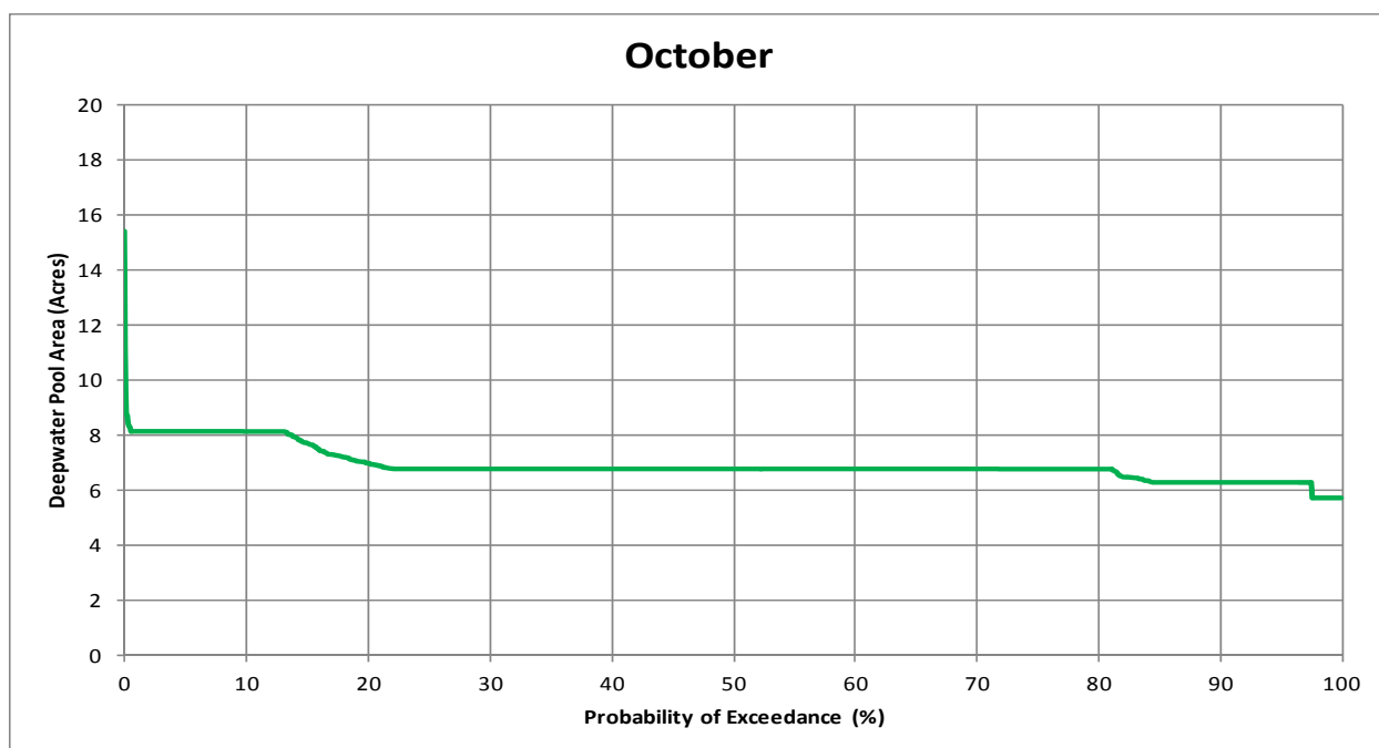
Figure 3.4-10. Simulated adult green sturgeon deepwater holding habitat exceedance during October for WY 1970 through 2010.
