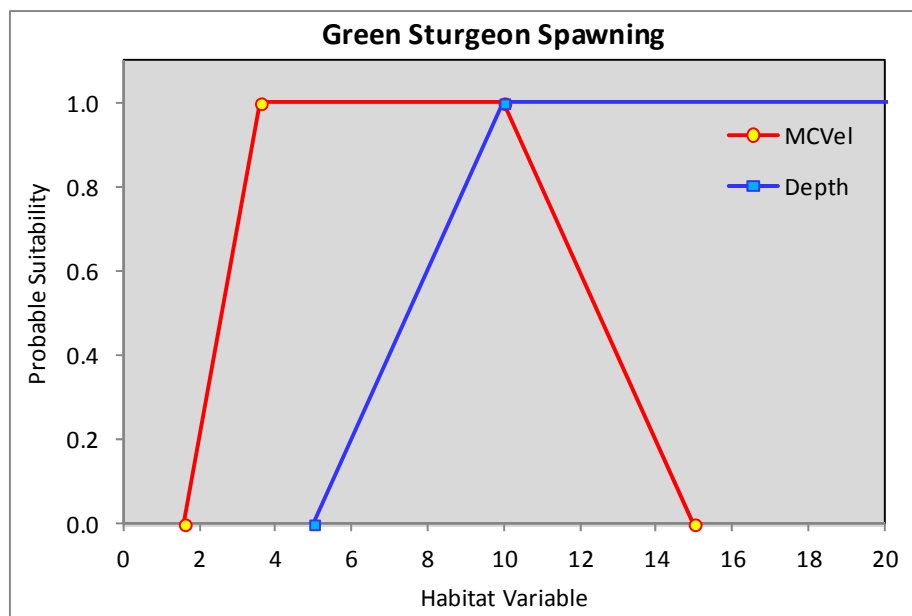
Figure 2.2-1. Green sturgeon spawning habitat suitability curves for water velocity and depth.
