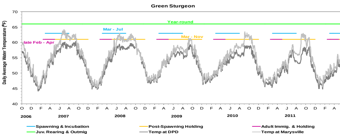
Figure 3.4-24. Monitored water temperatures and upper water temperature index value ranges for green sturgeon.
