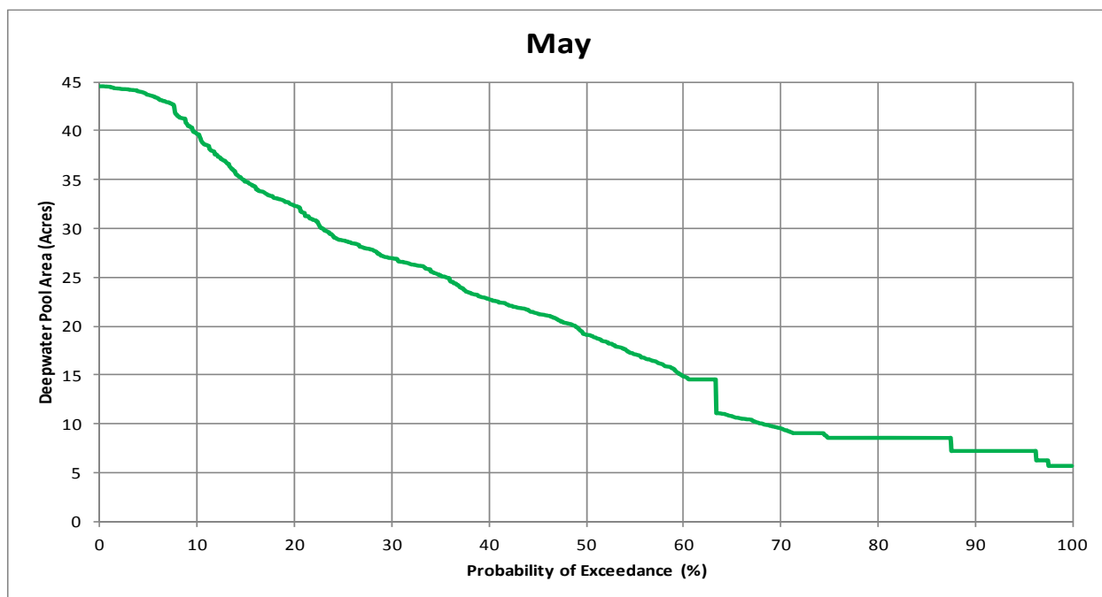
Figure 3.4-5. Simulated adult green sturgeon deepwater holding habitat exceedance during May for WY 1970 through 2010.
