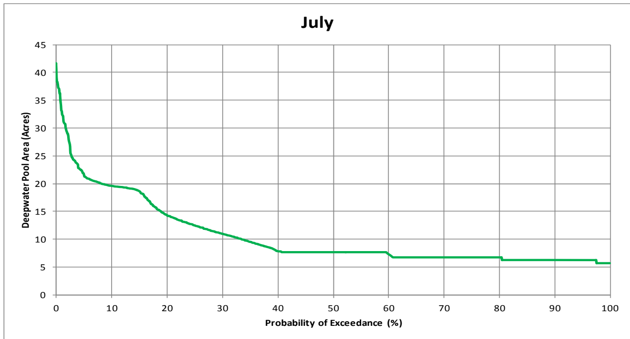
Figure 3.4-7. Simulated adult green sturgeon deepwater holding habitat exceedance during July for WY 1970 through 2010.
