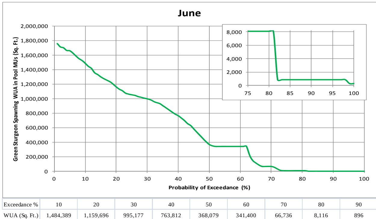
Figure 3.4-20. Simulated green sturgeon spawning WUA exceedance (in pool morphological units) during June for WY 1970 through 2010.
