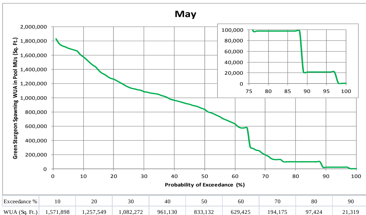
Figure 3.4-18. Simulated green sturgeon spawning WUA exceedance (in pool morphological units) during May for WY 1970 through 2010.
