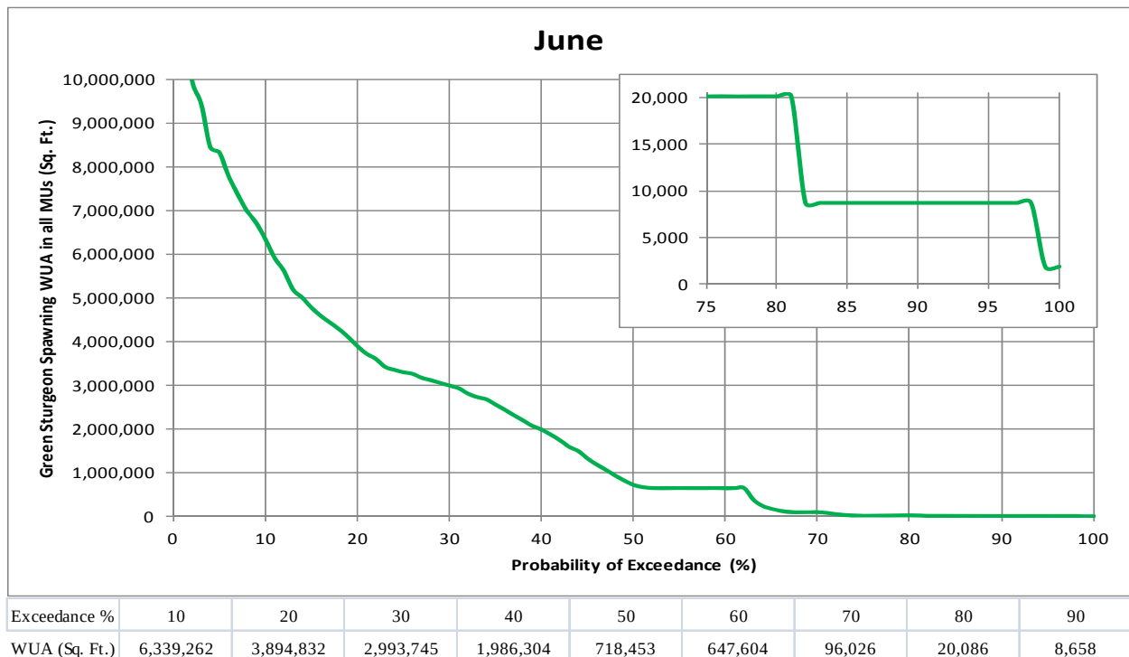
Figure 3.4-21. Simulated green sturgeon spawning WUA (in all morphological units) exceedance during June for water years 1970 through 2010.
