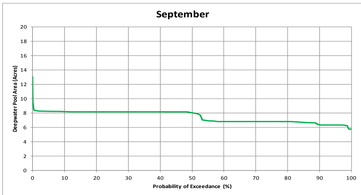
Figure 3.4-9. Simulated adult green sturgeon deepwater holding habitat exceedance during September for WY 1970 through 2010.
