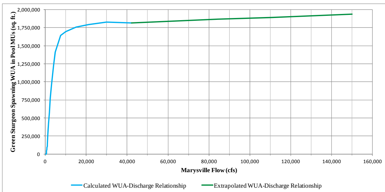
Figure 3.4-12. Relationship between flows at the Marysville Gage and green sturgeon spawning WUA (in pool morphological units) in the Yuba River downstream of Daguerre Point Dam.
