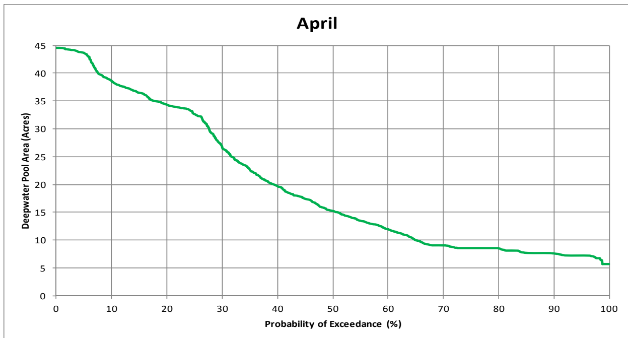
Figure 3.4-4. Simulated adult green sturgeon deepwater holding habitat exceedance during April for WY 1970 through 2010.
