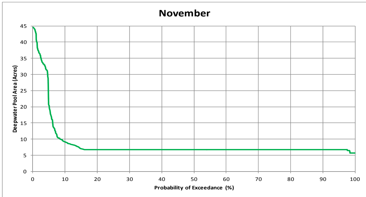
Figure 3.4-11. Simulated adult green sturgeon deepwater holding habitat exceedance during November for WY 1970 through 2010.
