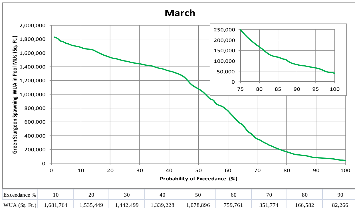
Figure 3.4-14. Simulated green sturgeon spawning WUA (in pool morphological units) exceedance during March for WY 1970 through 2010.
