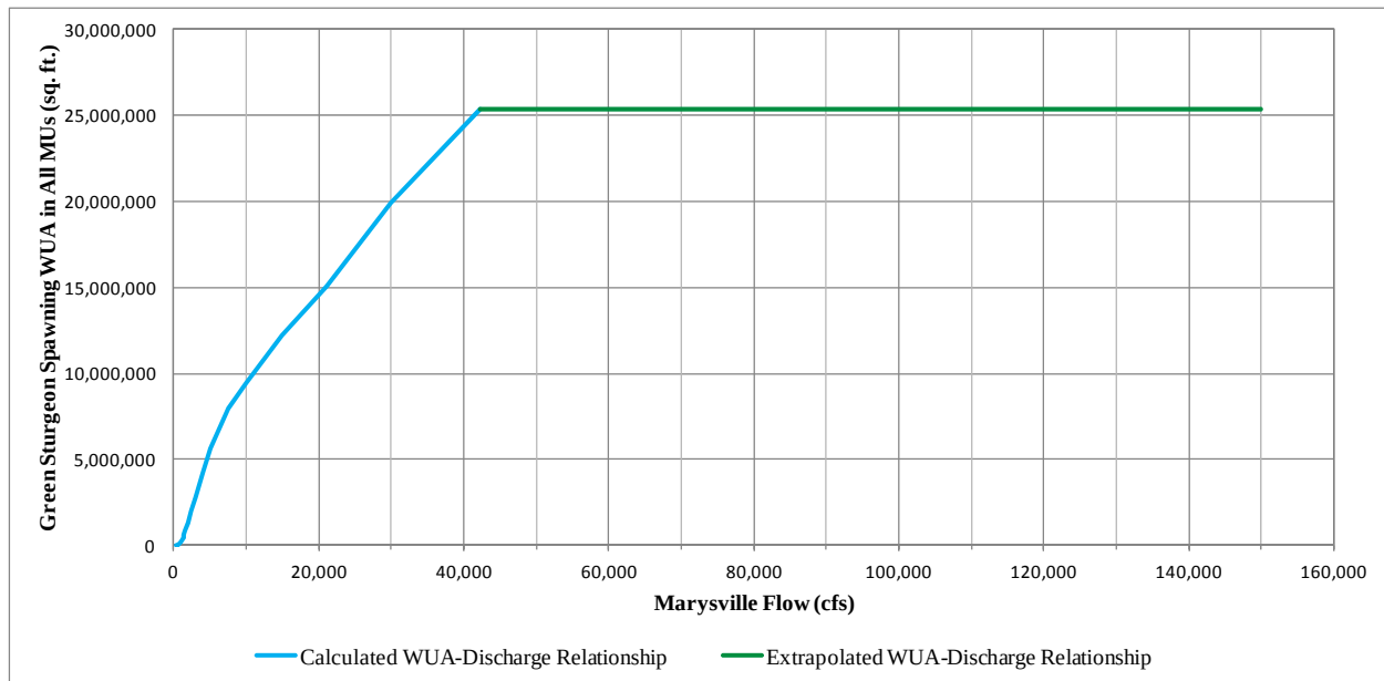
Figure 3.4-13. Relationship between flows at the Marysville Gage and green sturgeon spawning WUA (in all morphological units) in the Yuba River downstream of Daguerre Point Dam.
