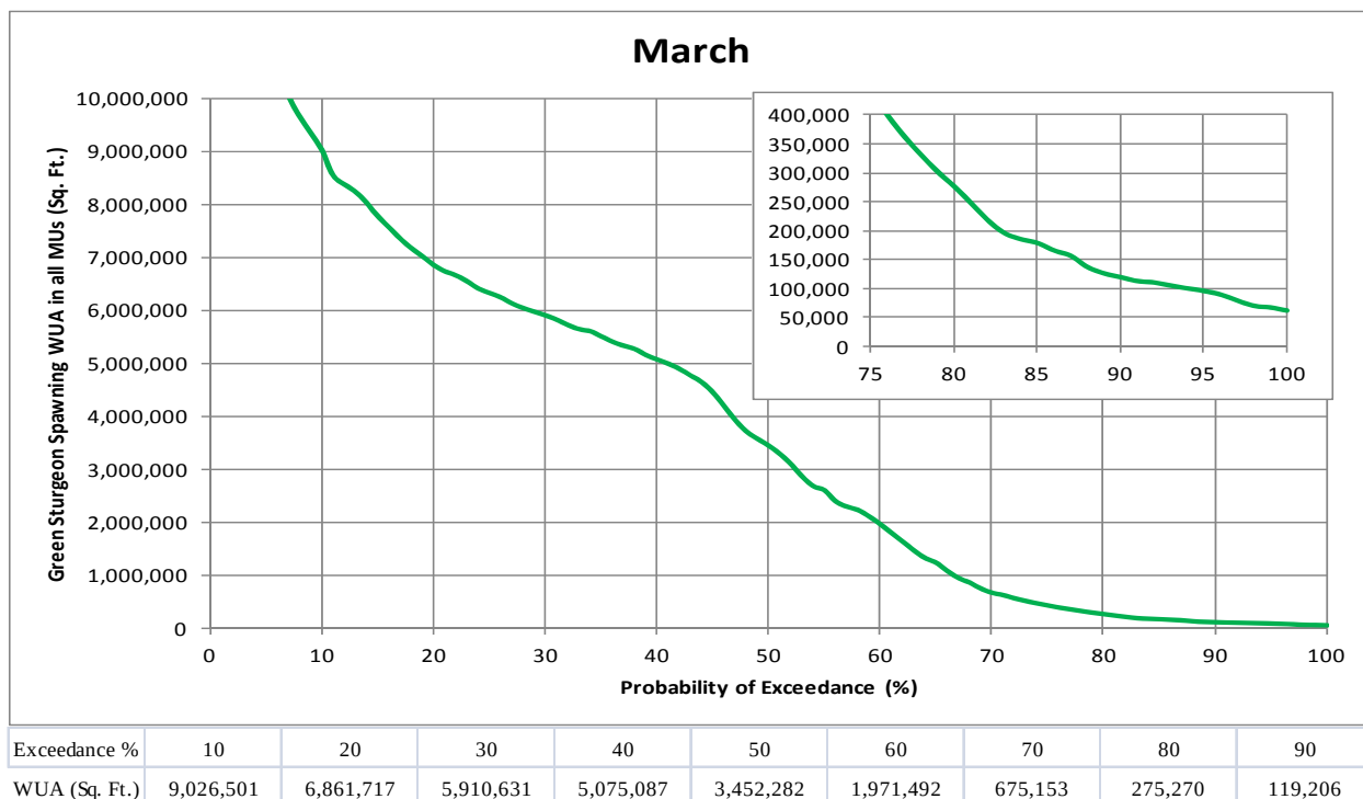
Figure 3.4-15. Simulated green sturgeon spawning WUA (in all morphological units) exceedance during March for WY 1970 through 2010.
