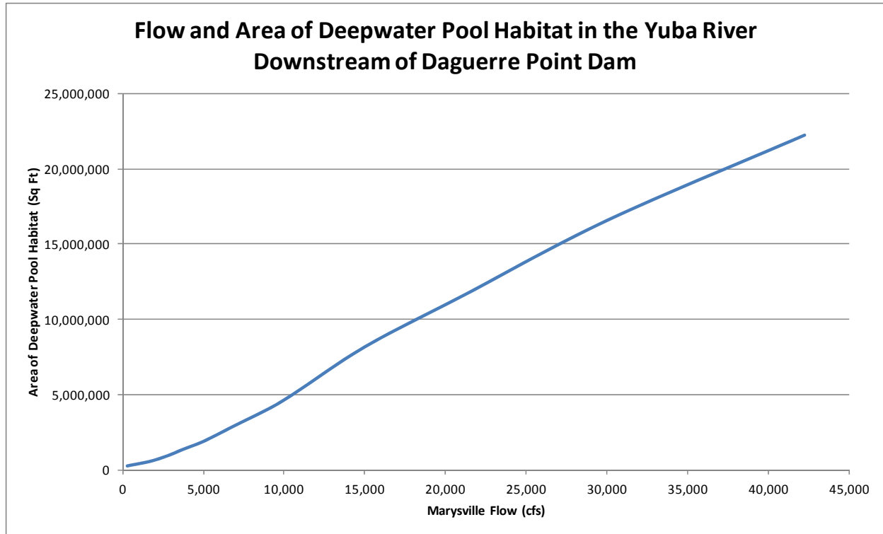
Figure 3.4-1. Marysville flows and areas of deepwater pool habitat in the Yuba River downstream of Daguerre Point Dam.
