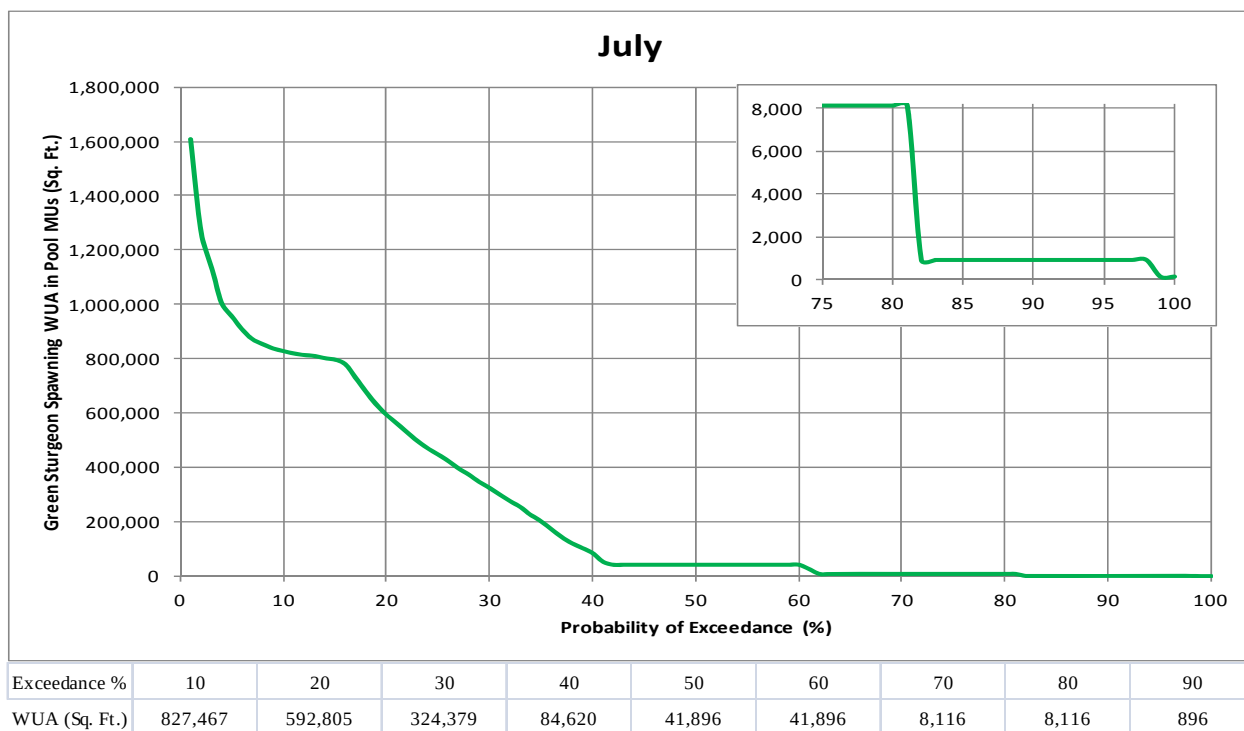
Figure 3.4-22. Simulated green sturgeon spawning WUA exceedance during July for WY 1970 through 2010.
