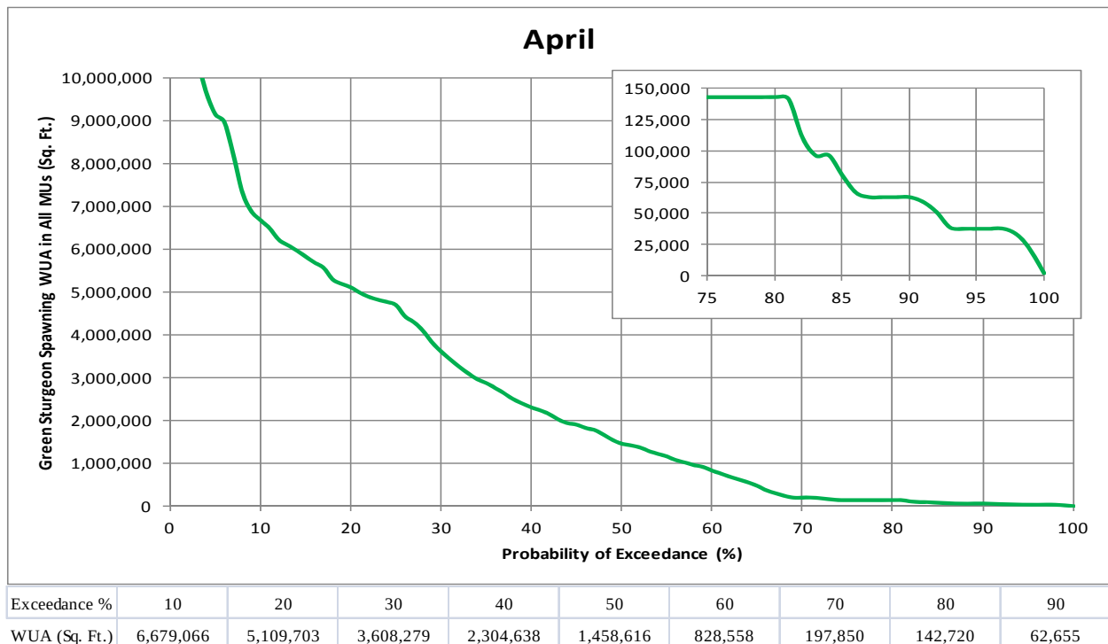
Figure 3.4-17. Simulated green sturgeon spawning WUA (in all morphological units) exceedance during April for WY 1970 through 2010.
