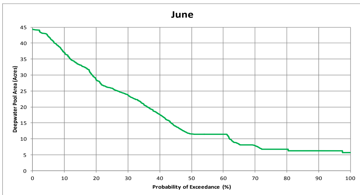
Figure 3.4-6. Simulated adult green sturgeon deepwater holding habitat exceedance during June for WY 1970 through 2010.
