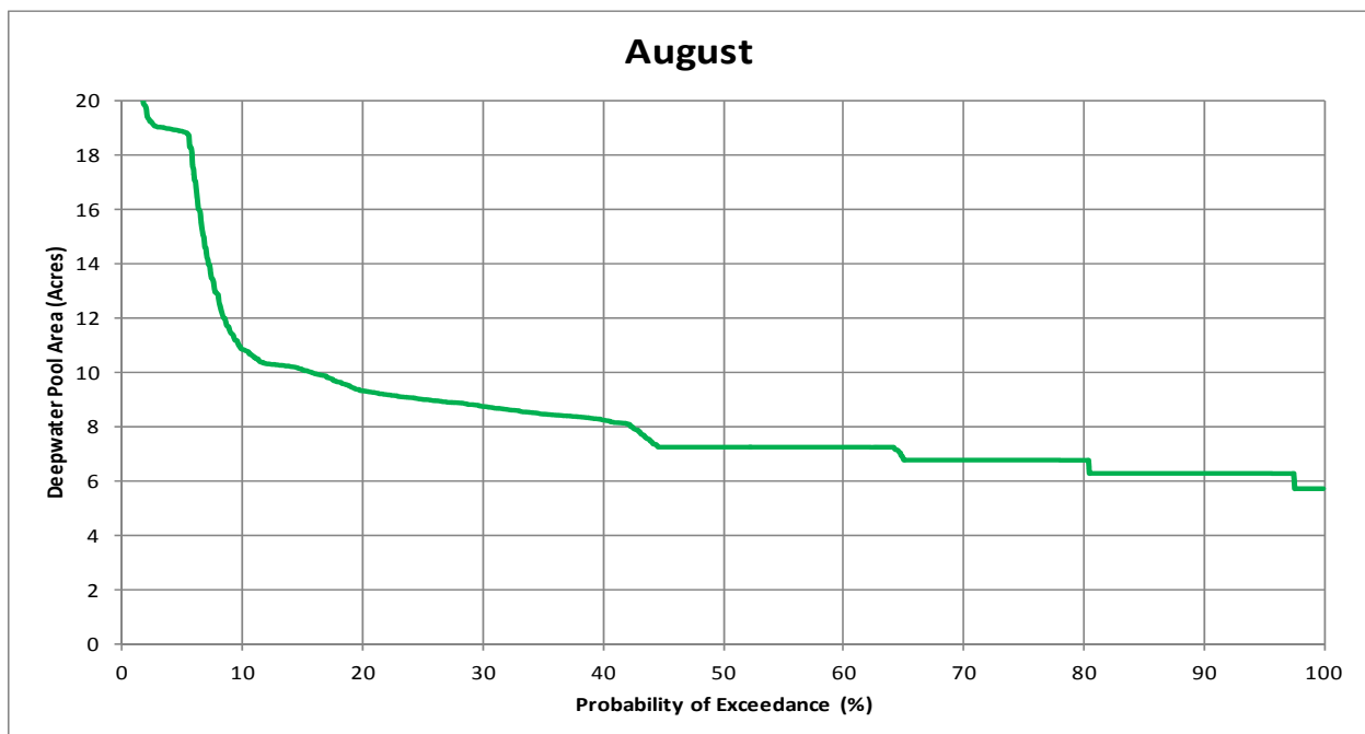
Figure 3.4-8. Simulated adult green sturgeon deepwater holding habitat exceedance during August for WY 1970 through 2010.
