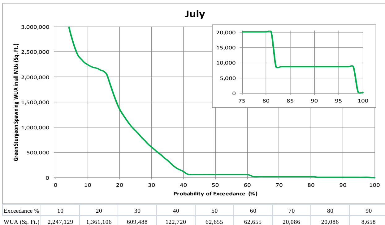
Figure 3.4-23. Simulated green sturgeon spawning WUA (in all morphological units) exceedance during July for WY 1970 through 2010.
