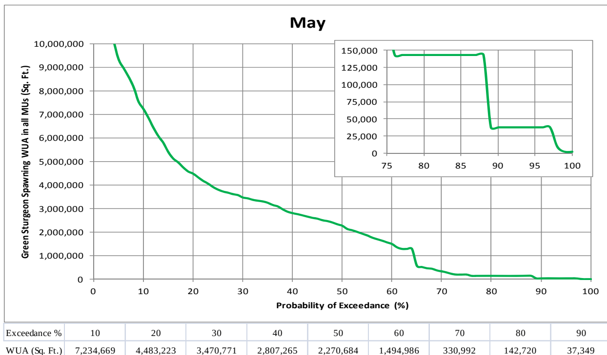
Figure 3.4-19. Simulated green sturgeon spawning WUA (in all morphological units) exceedance during May for WY 1970 through 2010.
